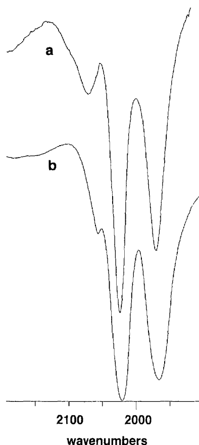
Fig. 4. (a) IR spectra (KBr pellets) of Rh/XGphtu* after three catalytic runs; (b) IR spectra (THF solution) of the thioureato complex [\text{Rh}(\text{CO})_2(\text{PhNC}(\text{S})\text{NHPh})] .
