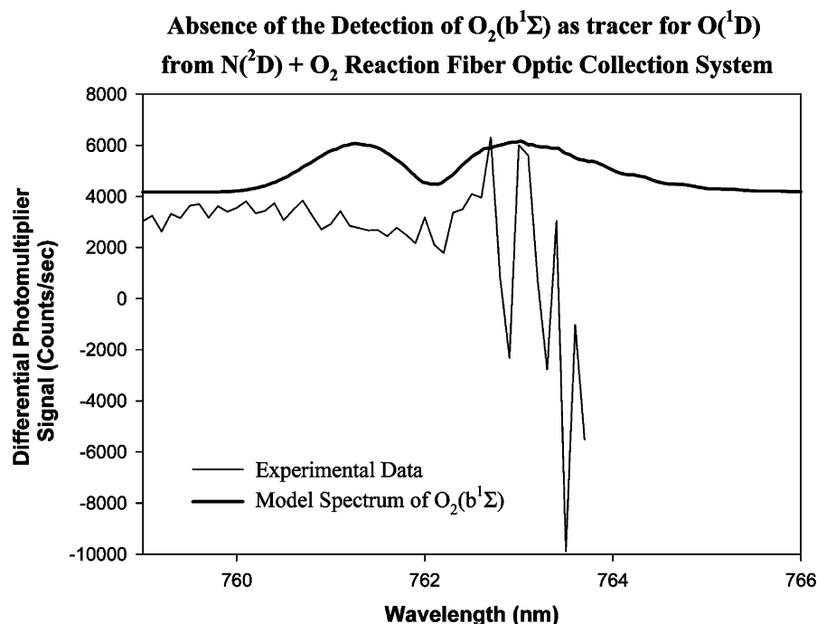
Figure 5. O 2 (b 1 Σ, v = 0) spectral region using fiber-optic collection. The experimental data curve is the difference between an averaged co-added set of monochromator scans with a pure O 2 counterflow and a scan with a pure argon counterflow (no in situ production of O( 1 D)/O 2 (b 1 Σ) possible). The calculated model spectrum of O 2 (b 1 Σ, v = 0) is shown for spectral reference. The larger noise at wavelengths >762.5 nm is due to the differential nature of the experimental curve (the difference of large numbers under the Ar line).
