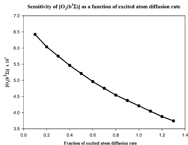
Figure 16. [O_2(b^1\Sigma)] dependence on diffusion rates. Diffusion rates from this figure were changed fractionally from the following values: O(^1D) , 442\text{ s}^{-1} ; N(^2D) , 570\text{ s}^{-1} ; and N(^2P) , 487\text{ s}^{-1} . Other conditions included a pressure of 4 mTorr, a temperature of 100 K, an N(^2D) mole fraction of 4 \times 10^{-5} , and a quench rate for O(^1D) by O_2 of 2.5 \times 10^{-11}\text{ cm}^3\text{ molecule}^{-1}\text{ s}^{-1} .
