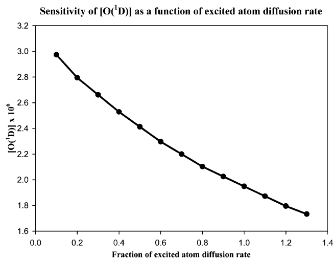
Figure 15. [O(^1D)] dependence on diffusion rates. Diffusion rates from this figure were changed fractionally from the following values: O(^1D) , 442\text{ s}^{-1} ; N(^2D) , 570\text{ s}^{-1} ; and N(^2P) , 487\text{ s}^{-1} . Other conditions included a pressure of 4 mTorr, a temperature of 100 K, an N(^2D) mole fraction of 4 \times 10^{-5} , and a quench rate for O(^1D) by O_2 of 2.5 \times 10^{-11}\text{ cm}^3\text{ molecule}^{-1}\text{ s}^{-1} .
