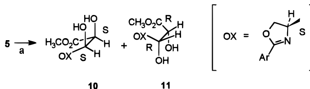
Scheme 4 a
