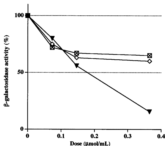
Figure 5. Suppression of UV-induced SOS response by 1 , 1A , and 1M in S. typhimurium TA1535/pSK1002: (▼) effect of 1 on UV irradiation; (crossed box) effect of 1A on UV irradiation; (◇) effect of 1M on UV irradiation.
