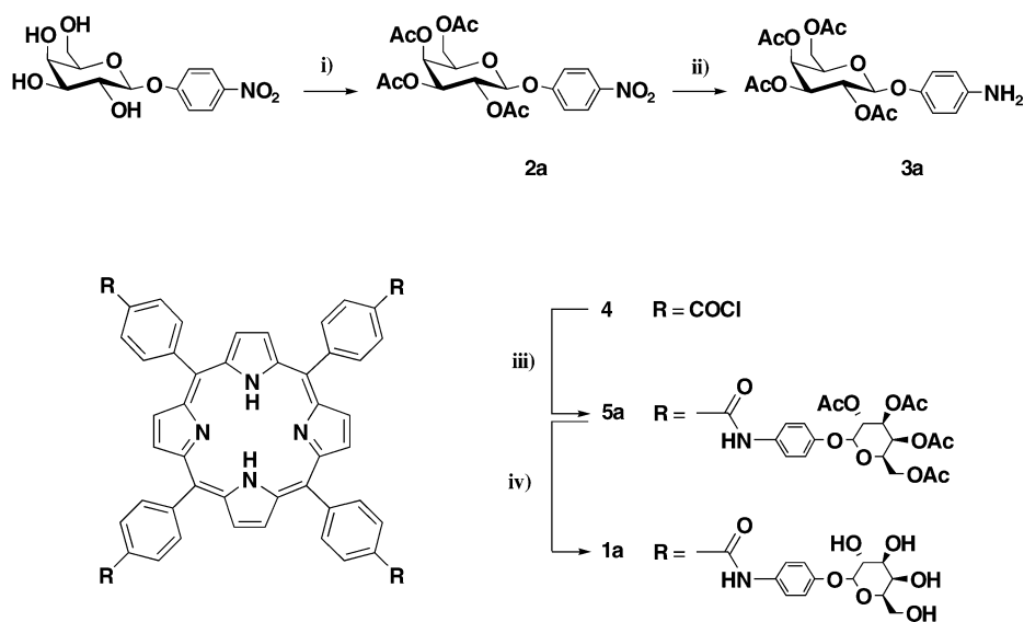
Scheme 2. Synthesis of the sugar-appended porphyrin 1a . Conditions: i) \text{Ac}_2\text{O} , pyridine; ii) \text{Pd/C} , \text{H}_2 , \text{AcOEt} ; iii) 3a , TEA, THF; iv) \text{CH}_3\text{ONa} , MeOH, THF. Compounds 1b – e are synthesized according to the same strategy.
