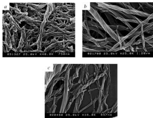
Figure 2. SEM images of the xerogels of a) 1a partial gel (DMF/benzylalcohol 1:3 (v/v), [ 1a ] = 4.0 \text{ g dm}^{-3} ), b) 1b gel (DMF/benzylalcohol 1:2 (v/v), [ 1b ] = 17 \text{ g dm}^{-3} ), and c) 1c gel (DMF/benzylalcohol 1:2 (v/v), [ 1c ] = 7.0 \text{ g dm}^{-3} ).
