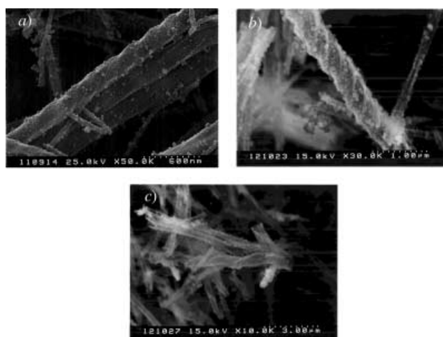
Figure 5. SEM images of the silica structure prepared by method B: a) 1a, b) 1b, and c) 1c gel fibrils as a template (before calcination).
