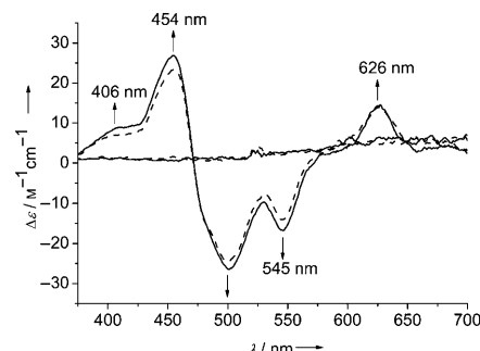
Figure 10. Solvent-dependent CD spectra of PBI-7 in MCH/CHCl 3 mixtures from 55:45 to 90:10 at a concentration of 1 × 10 −5 M in a 1 cm cuvette at 25°C. Arrows indicate the spectral changes with increasing amount of MCH.
