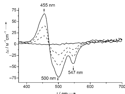
Figure 9. Solvent-dependent CD spectra of PBI-6 in MCH/CHCl 3 mixtures from 55:45 to 80:20 at a concentration of 1 × 10 −5 M at 25°C. Arrows indicate the spectral changes with increasing amount of MCH.
