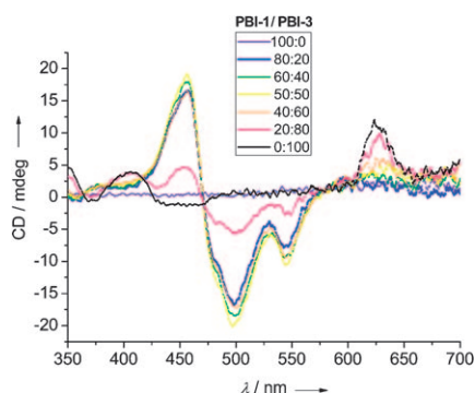
Figure 11. CD spectra of PBI-1 and PBI-3 in different ratios in MCH/ \text{CHCl}_3 mixtures (80:20) at 25°C. Total concentration of the chromophores were kept constant ( 1 \times 10^{-5} M) in each mixture.
