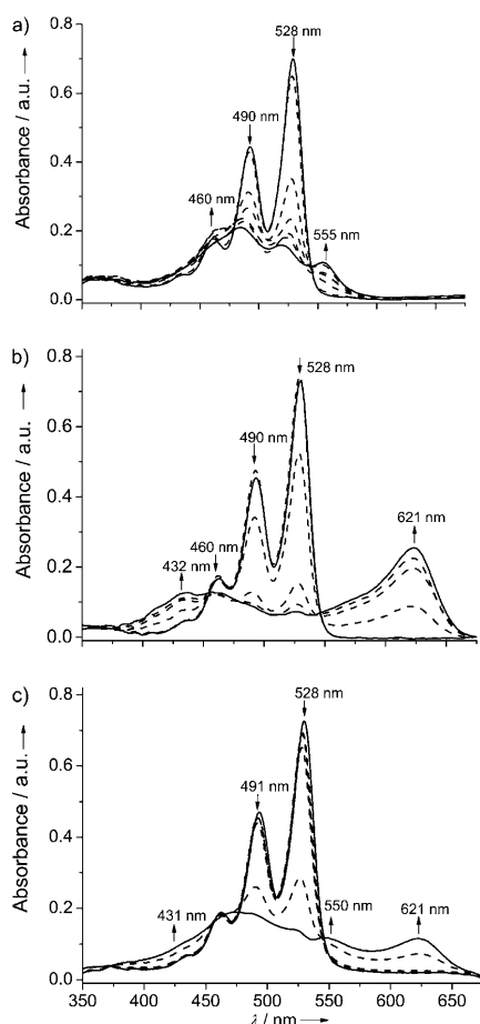
Figure 1. Solvent-dependent (in various MCH/ \text{CHCl}_3 mixtures) UV-visible absorption spectra of a) PBI-1 (50:50 to 80:20), b) PBI-4 (40:60 to 70:30), and c) PBI-7 (50:50 to 90:10) at a concentration of 1 \times 10^{-5} \text{ M} at 25^\circ\text{C} . Arrows indicate the spectral changes upon increasing the amount of MCH (from 40 to 90 %).
