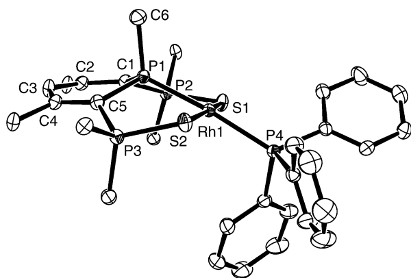
Figure 1. Molecular structure of 4 without hydrogen atoms. Phenyl groups of the phosphinine moiety have been omitted for clarity. Selected bond lengths (Å) and angles (deg): P1–Rh1 = 2.2428(6), S1–Rh1 = 2.3197(6), S2–Rh1 = 2.3213(6), P4–Rh1 = 2.3034(6); S1–Rh–S2 = 172.51(2), P1–Rh–P4 = 174.65(2), P1–C1–P2 = 113.6(1), P1–C5–P3 = 111.1(1), (mean plane C1–C2–C4–C5)–P1 = 16.7, (mean plane C1–C2–C4–C5)–C3 = 7.1, S1–P2–C1–P1 = 4.3, S2–P3–C5–P1 = 13.0.
