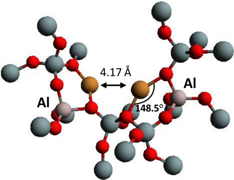
Figure 9. Structural model for the binuclear CuI precursor (in yellow) of the Cu-O-Cu site in ZSM-537. Si atoms are in gray and oxygen atoms in red. 43x34mm (600 x 600 DPI)
