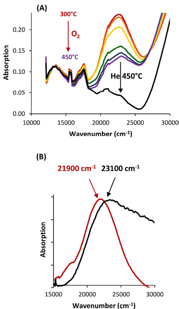
Figure 2. (A) Intensity decrease upon heating a Cu-MOR sample in \text{O}_2 flow to 450^{\circ}\text{C} after \text{O}_2 activation at 250^{\circ}\text{C} , the spectra are measured at respectively 300^{\circ}\text{C} (red), 330^{\circ}\text{C} (orange), 360^{\circ}\text{C} (yellow), 390^{\circ}\text{C} (green), 420^{\circ}\text{C} (blue) and 450^{\circ}\text{C} (purple). The spectrum after complete autoreduction in helium flow at 450^{\circ}\text{C} is shown in black; (B) difference of two consecutive spectra during heating in \text{O}_2 to 450^{\circ}\text{C} (red) and the difference between the spectrum measured in \text{O}_2 at 450^{\circ}\text{C} and \text{He} at 450^{\circ}\text{C} (black).
