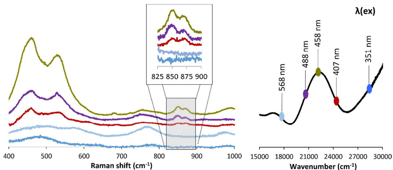
Figure 6. Resonance Raman spectra of \text{N}_2\text{O} -activated Cu-MOR collected at various excitation energies (left). Note the shift in relative intensity of the features between 825\text{--}900\text{ cm}^{-1} (left). The different laser excitation lines (in nm) are indicated on the absorption spectrum of an \text{O}_2 activated MOR (right).
