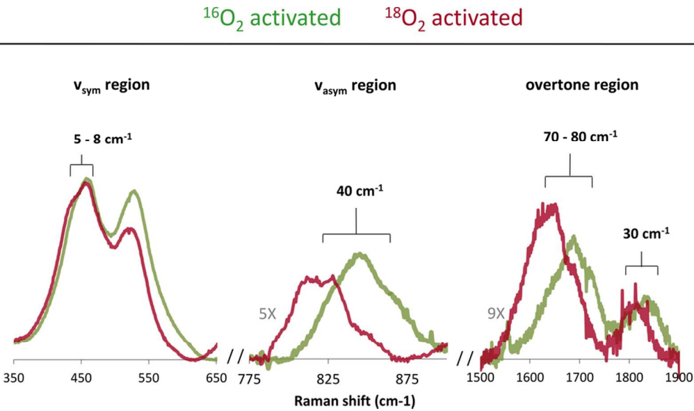
Figure 7. Resonance Raman spectra ( \lambda_{\text{ex}}=458\text{ nm} ) of Cu-MOR activated with ^{18}\text{O}_2 (red) and subsequent ^{16}\text{O}_2 activation (green). 91x52mm (300 x 300 DPI)
