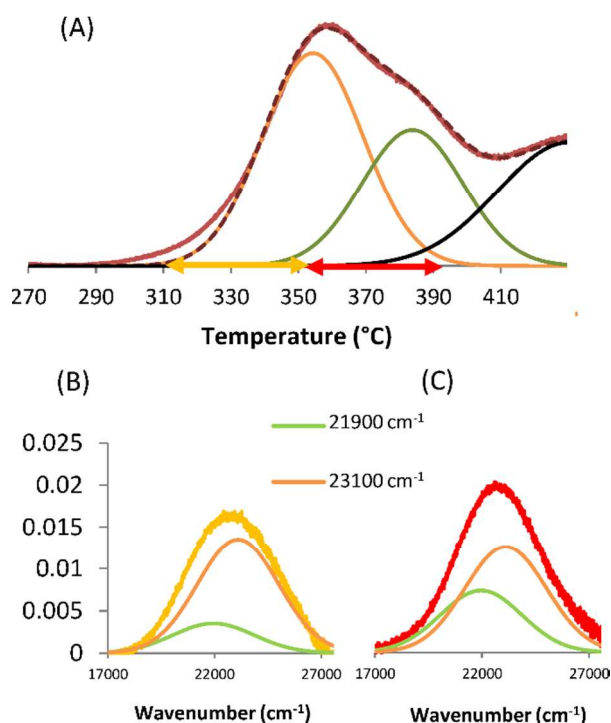
Figure 3. (A) MS signal of \text{O}_2 during TPD of an activated Cu-MOR (red) and its fitted peaks (dashed line is the sum), (B) Difference spectrum between absorption spectra at 310^\circ\text{C} and 350^\circ\text{C} and (C) difference spectrum between absorption spectra at 350^\circ\text{C} and 390^\circ\text{C} , deconvoluted with absorption maxima at 21900\text{ cm}^{-1} and 23100\text{ cm}^{-1} .
