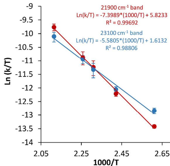
Figure 4. Eyring Kinetics of \text{CH}_4 Reaction with Activated Cu-MOR. Eyring plots derived from the decay of Cu-MOR's deconvolution bands at 23100 \text{cm}^{-1} (blue) and 21900 \text{cm}^{-1} (red) during reaction with \text{CH}_4 . Error bars indicate the 95% confident interval of the linear regression.
