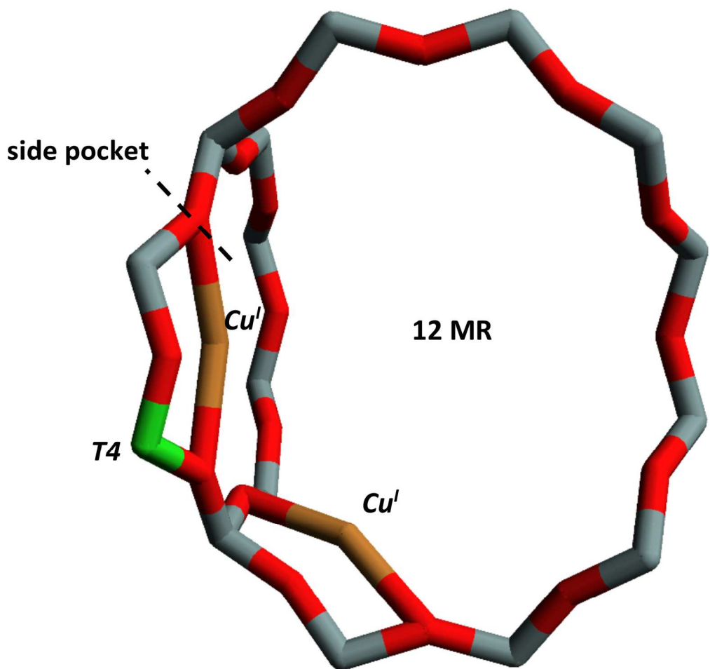
Figure S6. CuI ions bound bidentate with bite angles of 150^\circ can be placed at two positions (in yellow) in the 12 MR. 85x80mm (600 x 600 DPI)
