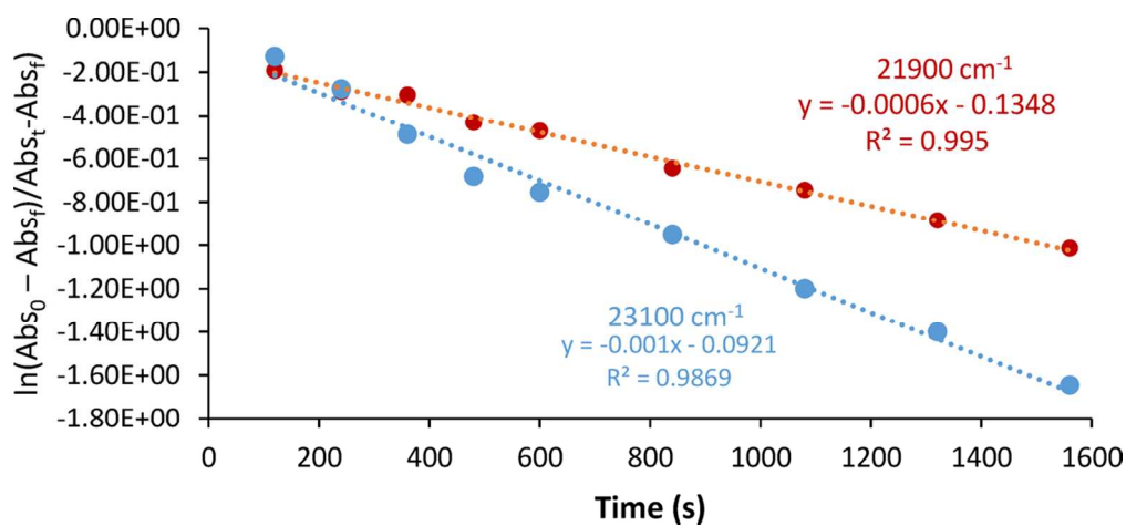
Figure S3. First order plots of the decay of the 21900 and 23100 cm -1 bands at 110°C. 52x24mm (600 x 600 DPI)
