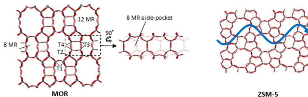
Figure 10. Framework structures of mordenite (left) and ZSM-5 (right). Si atoms are in grey and O atoms are in red. The four non-equivalent tetrahedral sites of mordenite are indicated on the structure. The blue arrow indicates the sinusoidal 10 MR channel in ZSM-5.
