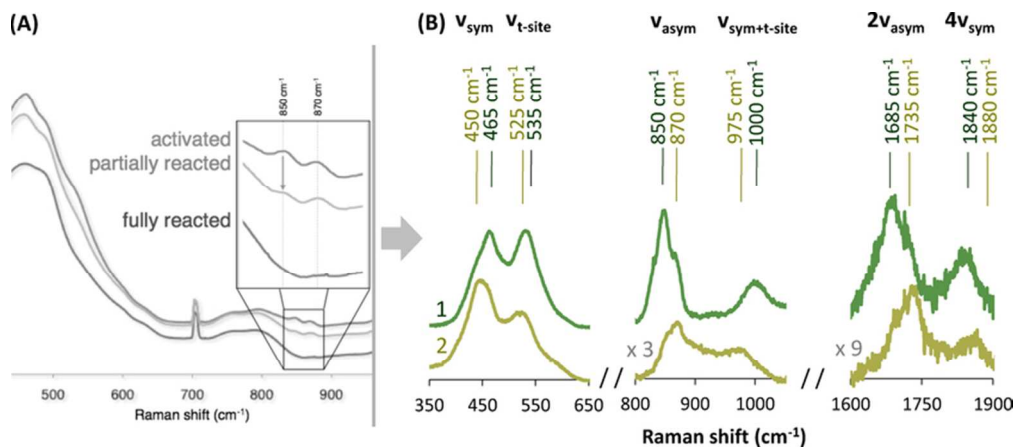
Figure 8. (A) Resonance Raman spectra ( \lambda_{\text{ex}}=458 nm) of activated Cu-MOR during reaction with CH 4 at 200 °C. Note the relative decrease of the 850 cm -1 vibration after partial reaction. (B) rR spectra of individual MOR sites 1 (green) and 2 (yellow) generated by subtraction of spectra from activated and partially reacted samples ( \lambda_{\text{ex}}=458 nm). 71x30mm (300 x 300 DPI)
