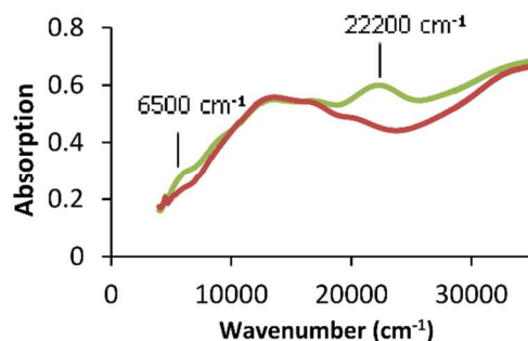
Figure 1. Cu-MOR sample after O 2 activation at 250°C (green) and after subsequent methane reaction at 150°C (red).
