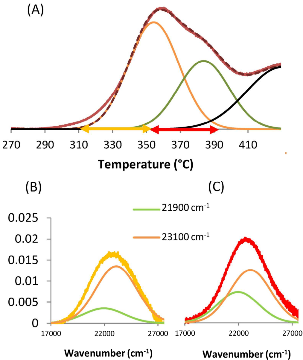
Figure 3. (A) MS signal of O 2 during TPD of an activated Cu-MOR (red) and its fitted peaks (dashed line is the sum), (B) Difference spectrum between absorption spectra at 310°C and 350° and (C) difference spectrum between absorption spectra at 350°C and 390°C, deconvoluted with absorption maxima at 21900 cm -1 and 23100 cm -1 . 93x110mm (600 x 600 DPI)
