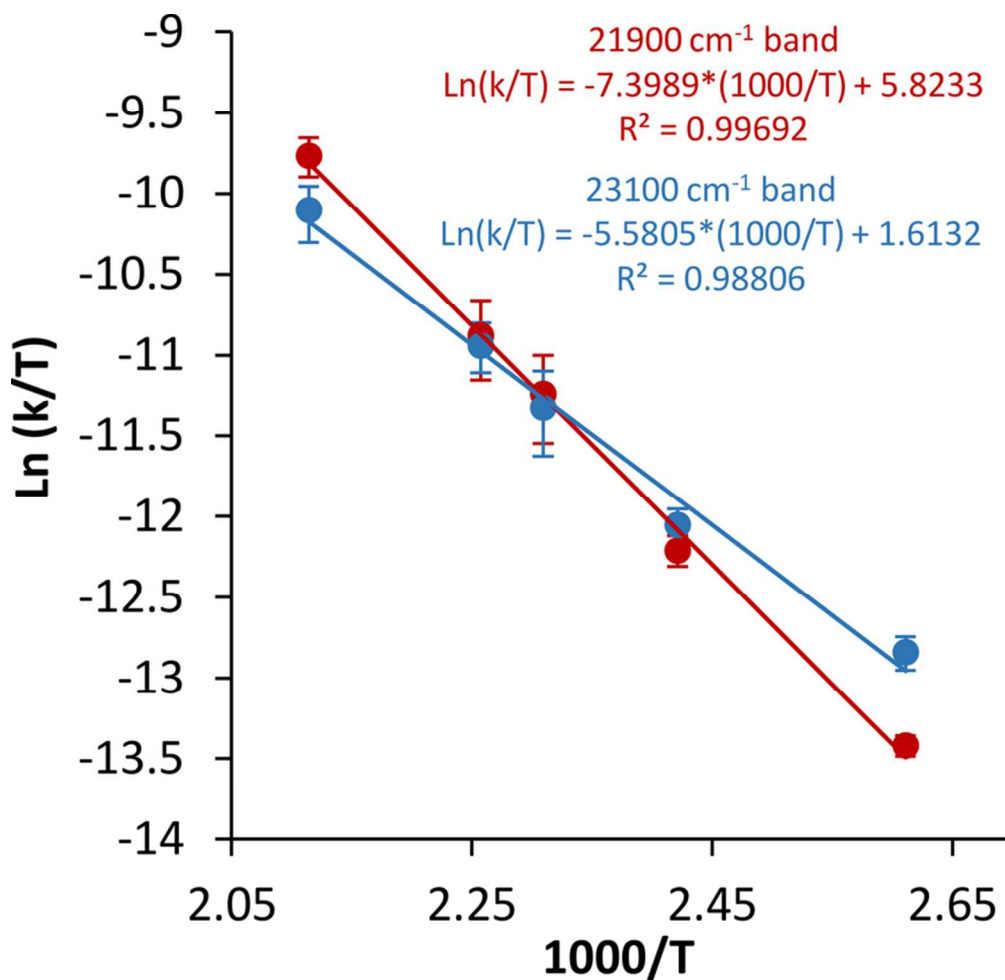
Figure 4. Eyring Kinetics of CH 4 Reaction with Activated Cu-MOR. Eyring plots derived from the decay of Cu-MOR's deconvolution bands at 23100 cm -1 (blue) and 21900 cm -1 (red) during reaction with CH 4 . Error bars indicate the 95% confident interval of the linear regression. 73x71mm (300 x 300 DPI)
