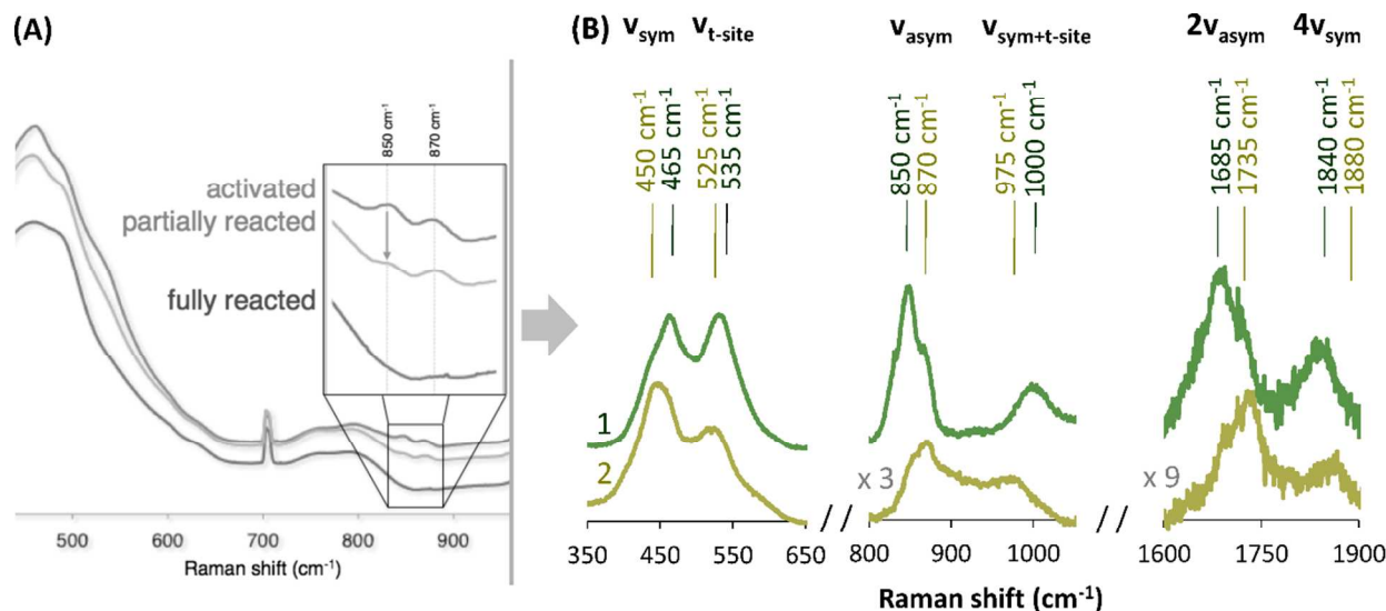
Figure 8. (A) Resonance Raman spectra ( \lambda_{\text{ex}}=458 nm) of activated Cu-MOR during reaction with \text{CH}_4 at 200 °C. Note the relative decrease of the 850\text{ cm}^{-1} vibration after partial reaction. (B) rR spectra of individual MOR sites 1 (green) and 2 (yellow) generated by subtraction of spectra from activated and partially reacted samples ( \lambda_{\text{ex}}=458 nm).
