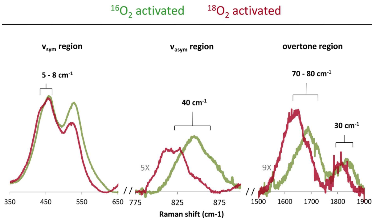
Figure 7. Resonance Raman spectra ( \lambda_{\text{ex}}=458 nm) of Cu-MOR activated with ^{18}\text{O}_2 (red) and subsequent ^{16}\text{O}_2 activation (green).
