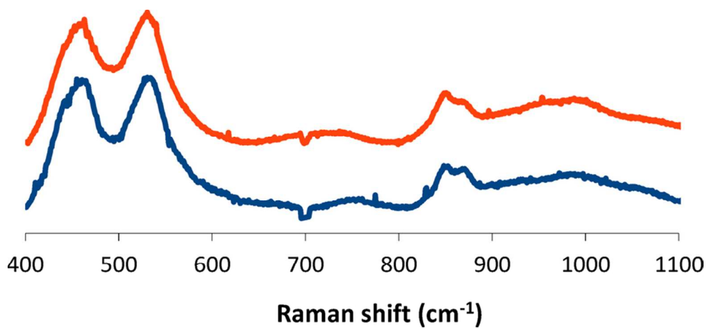
Figure S5. Resonance Raman spectra ( \lambda_{\text{ex}}=458 nm) of Cu-MOR activated with O 2 (red) and N 2 O (blue) at 250 °C. 41x18mm (600 x 600 DPI)
