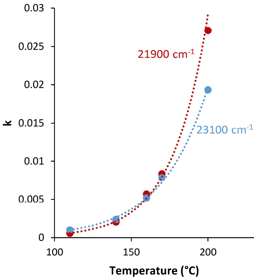
Figure S4. Comparison of the disappearance of the 21900 and 23100 cm -1 bands during the CH 4 reaction: k in function of the temperature. 76x83mm (600 x 600 DPI)
