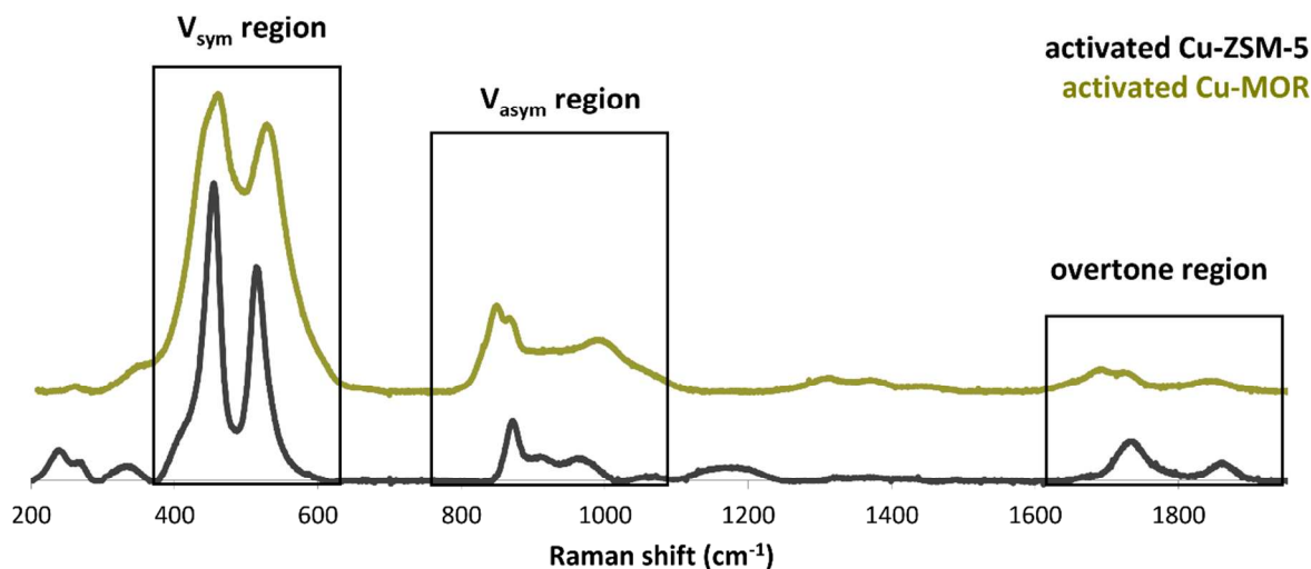
Figure 5. Comparison of the resonance Raman spectra ( \lambda_{\text{ex}}=458 nm) of \text{O}_2 activated Cu-MOR and Cu-ZSM-5.
