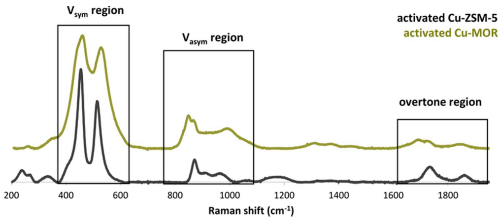
Figure 5. Comparison of the resonance Raman spectra ( \lambda_{\text{ex}}=458 nm) of O 2 activated Cu-MOR and Cu-ZSM-5. 65x28mm (300 x 300 DPI)
