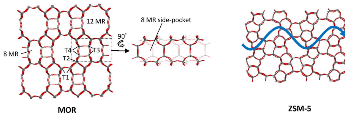
Figure 10. Framework structures of mordenite (left) and ZSM-5 (right). Si atoms are in grey and O atoms are in red. The four non-equivalent tetrahedral sites of mordenite are indicated on the structure. The blue arrow indicates the sinusoidal 10 MR channel in ZSM-5.
