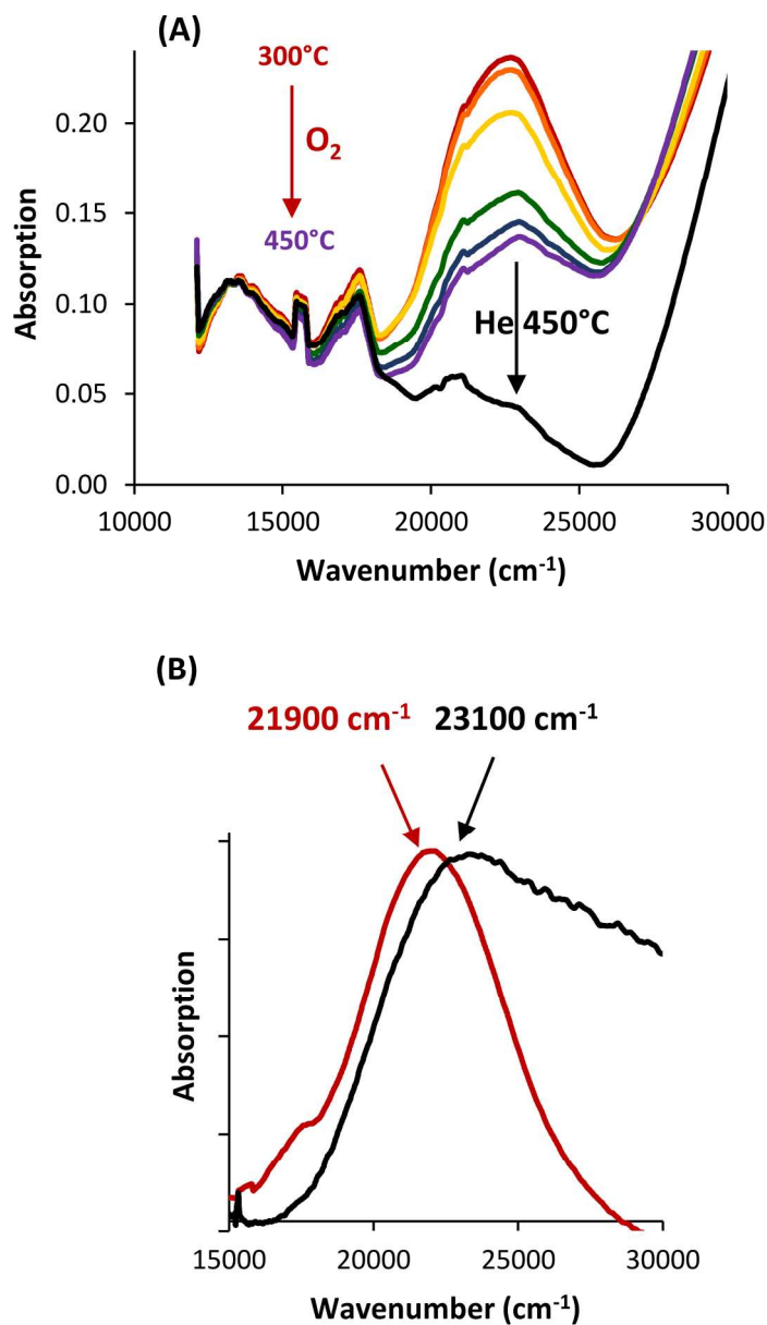
Figure 2. (A) Intensity decrease upon heating a Cu-MOR sample in O 2 flow to 450°C after O 2 activation at 250°C, the spectra are measured at respectively 300°C (red), 330°C (orange), 360°C (yellow), 390°C (green), 420°C (blue) and 450°C (purple). The spectrum after complete autoreduction in helium flow at 450°C is shown in black; (B) difference of two consecutive spectra during heating in O 2 to 450°C (red) and the difference between the spectrum measured in O 2 at 450°C and He at 450°C (black). 140x245mm (300 x 300 DPI)
