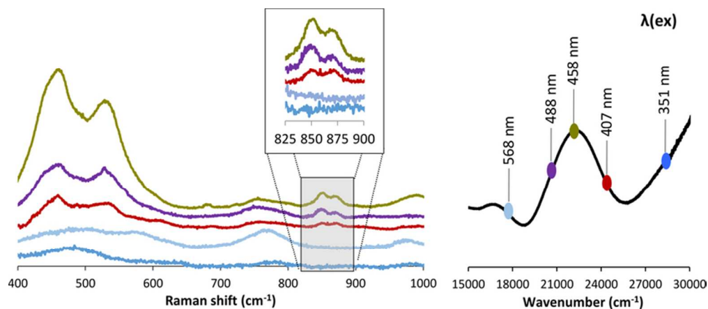
Figure 6. Resonance Raman spectra of N 2 O-activated Cu-MOR collected at various excitation energies (left). Note the shift in relative intensity of the features between 825-900 cm -1 (left). The different laser excitation lines (in nm) are indicated on the absorption spectrum of an O 2 activated MOR (right). 72x31mm (300 x 300 DPI)
