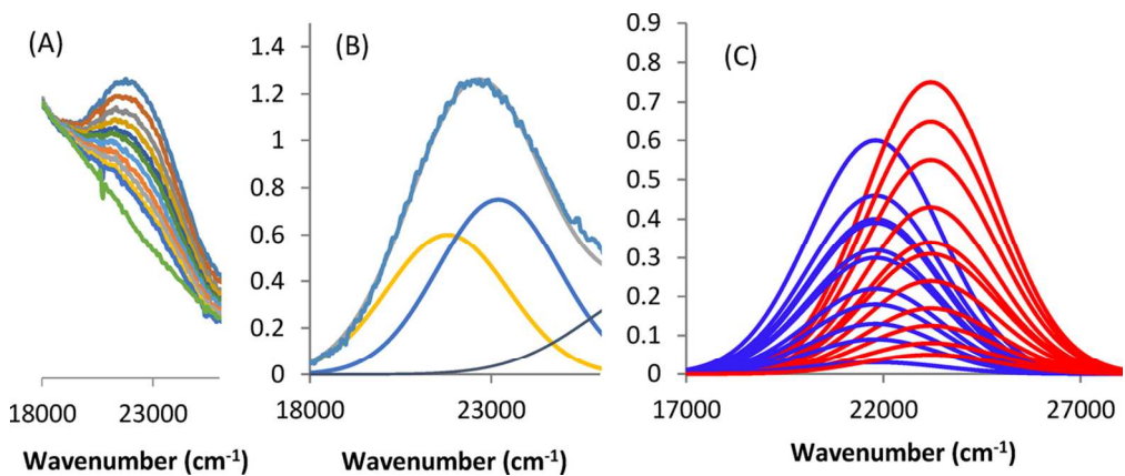
Figure S2. (A)Example of the disappearance of the 22200 cm-1 band envelope during CH4 reaction at 110°C; (B) Deconvolution of the absorption envelope at the start of the reaction. This is done for every spectrum that is measured in time. (C) The 21900 cm-1 and 23100 cm-1 absorption bands during CH4 reaction at 110°C 53x22mm (600 x 600 DPI)
