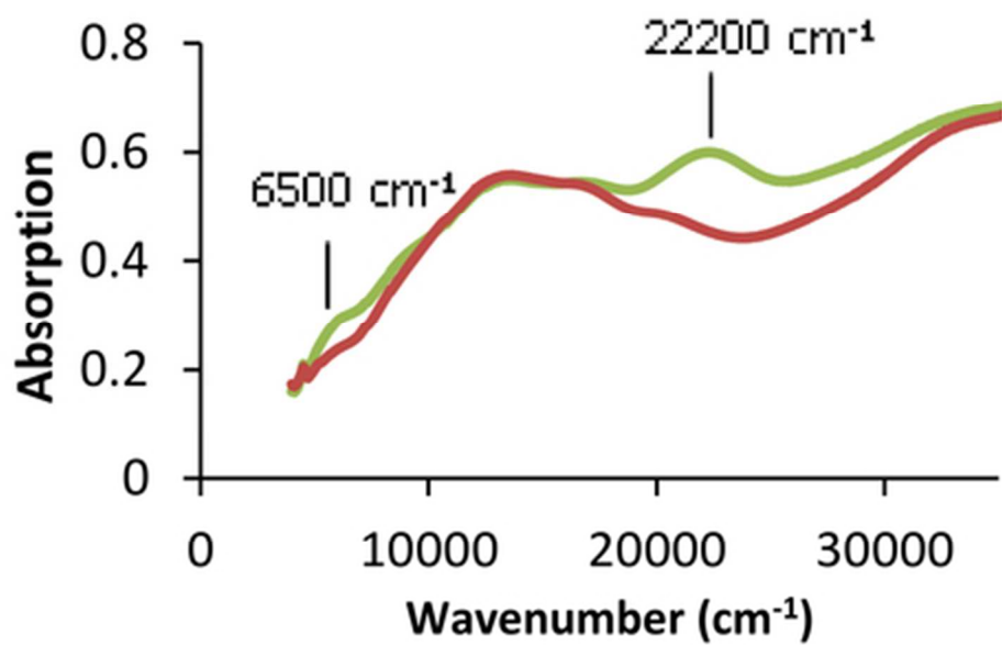
Figure 1. Cu-MOR sample after O 2 activation at 250°C(green) and after subsequent methane reaction at 150°C (red). 41x25mm (300 x 300 DPI)
