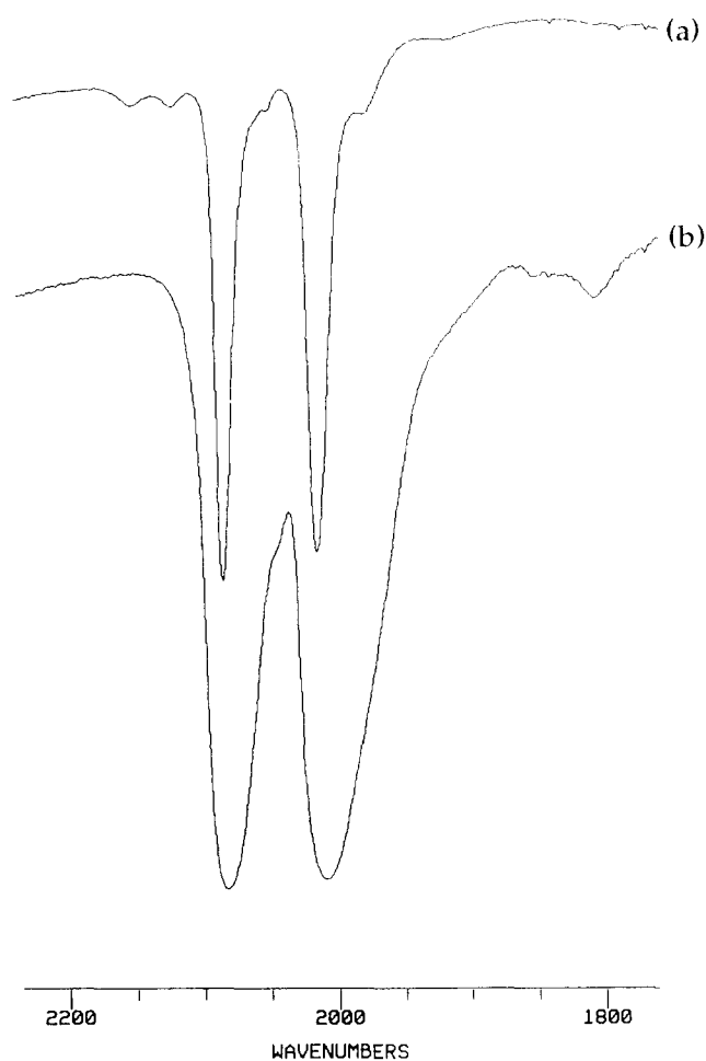
Fig. 1. Comparison between the IR spectra, in the carbonyl stretching region, of (a) the \text{Rh}(\text{CO})_2\text{Cl}/\text{Hbztu} complex in dichloromethane solution (2087, 2018 \text{cm}^{-1} ) and (b) the corresponding anchored species on XGhztu* (2083, 2010 \text{cm}^{-1} ).
