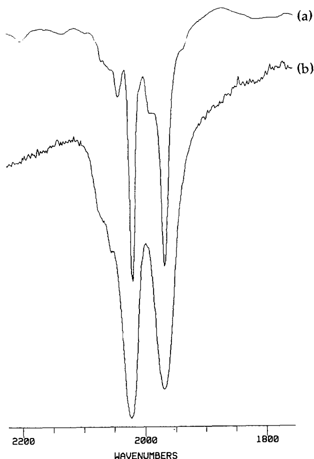
Fig. 2. Comparison between the IR spectra, in the carbonyl stretching region, of (a) the \text{Rh}(\text{CO})_2 /thiourea complex in tetrahydrofuran solution (2020, 1968 \text{cm}^{-1} ) and (b) the \text{Rh}/\text{XGbztu}^* catalyst after three cycles (2023, 1969 \text{cm}^{-1} ).
