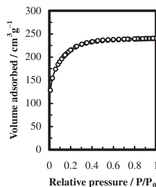
Figure 1. N 2 adsorption and desorption isotherm of the silica formed in the presence of 1.31 g of gelatin (Gel. 4) after being calcined at 500 °C in N 2 followed by O 2 . The isotherm was collected on a Micromeritics Tristar Analyzer after the sample was degassed at 150 °C for 12 h.
