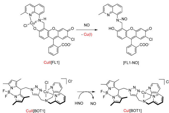
Scheme 1. Small-Molecule Metal-Containing Sensors for NO (Cu[FL1]) and HNO (Cu[BOT1]) as Well as Their Reactions with Analytes 30,33
