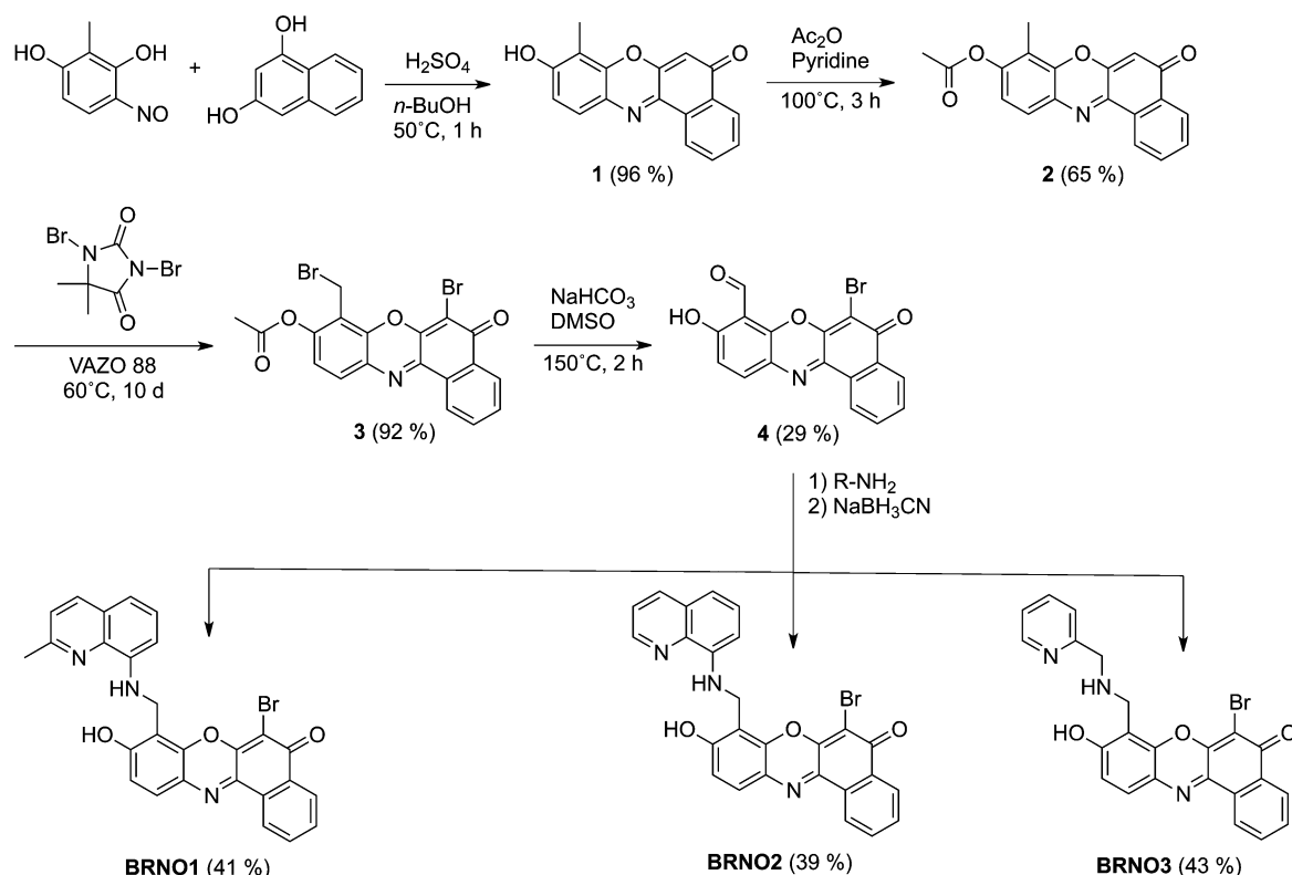
Scheme 2. Synthetic Scheme for the Synthesis of Benzoessorufin-Based Sensors BRNO1–3
