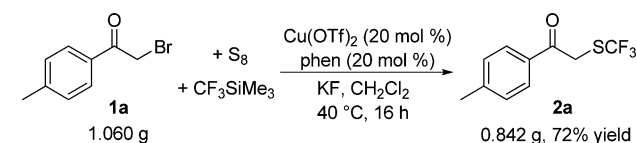
Scheme 4. Gram-Scale Synthesis of \alpha -Trifluoromethylthio-Substituted Ketones
