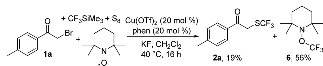
Scheme 6. Inhibition Experiment with TEMPO
