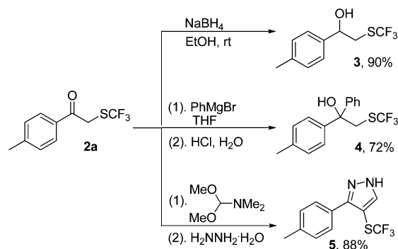
Scheme 5. Synthetic Utility of 2a
