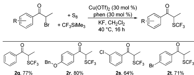
Scheme 3. Copper-Catalyzed Trifluoromethylthiolation of Secondary \alpha -Bromoketones a
