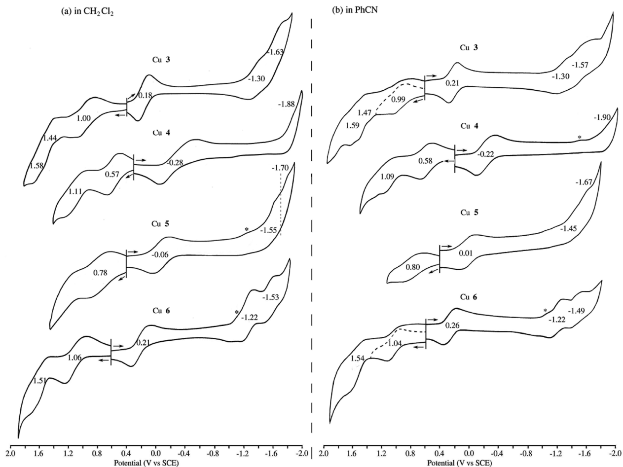
Figure 4. Cyclic voltammograms of (TBC)Cu derivatives ( 3–6 ) in \text{CH}_2\text{Cl}_2 and PhCN containing 0.2 M TBAP at scan rate of 0.1 V/s. Some small reduction peaks, marked by asterisks, are probably due to unstable reduced products.
