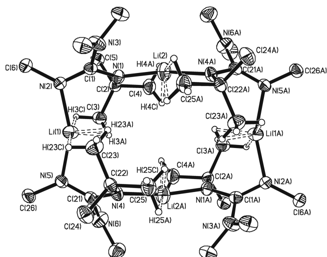
Figure 2. Diagram showing the molecular structures of the tetrameric lithium guanidinate complex 1c (50% probability ellipsoids). Hydrogen atoms on methyl groups not involved in supporting Li...H-C interactions and methyl carbons attached to C(6), C(26), C(6A), and C(26A) have been omitted for clarity. Symmetry transformations used to generate equivalent atoms: -x, y, 1/2 - z .
