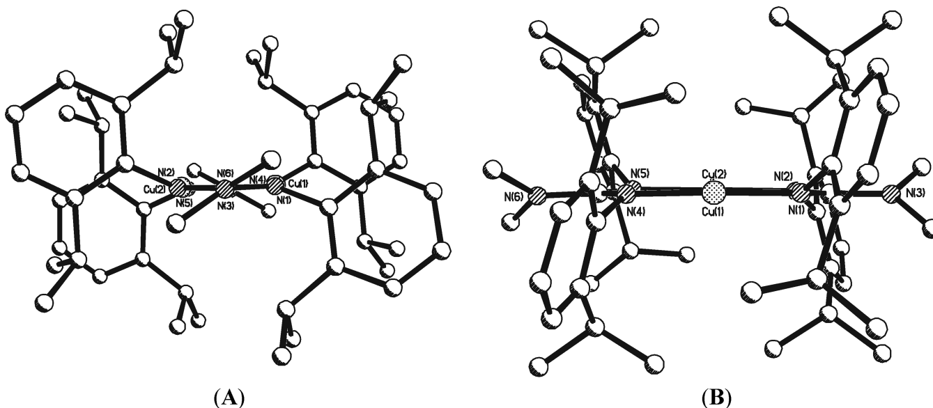
Figure 7. Views of the complex 2d down the N(3)–N(6) (A) and Cu(1)–Cu(2) (B) vectors respectively, highlighting the relative planarity of the central \{\text{Cu}_2\text{N}_4\text{C}_4\} core and the lack of twisting of the guanidinate about the Cu–Cu bond.
