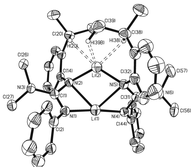
Figure 5. Diagram showing the molecular structures of the dimeric lithium guanidinate complex 1d (50% probability ellipsoids). Hydrogen atoms not involved in supporting Li...H-C interactions and isopropyl groups {CHMe 2 } attached to C(3), C(7), C(19), C(37), C(45), and C(49) have been omitted for clarity.
