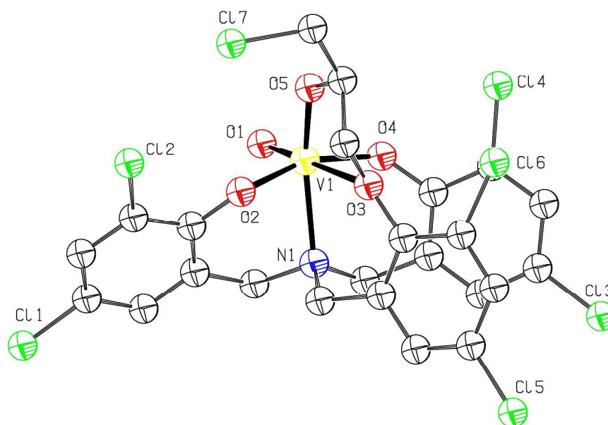
Figure 5. X-ray molecular structure of 2 -ECH based on V(V) complex 2 , ECH = epichlorohydrin. Selected bond lengths (Å) and angles (°), with esd's in parentheses: V(1)-O(1) = 1.585(4), V(1)-O(2) = 1.893(4), V(1)-O(3) = 2.327(4), V(1)-O(4) = 1.879(4), V(1)-O(5) = 1.808(4), V(1)-N(1) = 2.233(5); O(4)-V(1)-N(1) = 84.25(17), O(1)-V(1)-O(3) = 179.8(2), O(2)-V(1)-O(5) = 92.21(19), O(2)-V(1)-O(4) = 159.53(18), N(1)-V(1)-O(5) = 156.53(19).
