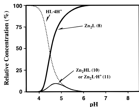
Figure 2. Distribution diagram for the zinc(II) species in 5 mM propanol-bridged octaazacryptand 7/10 mM zinc(II) system as a function of pH at 35 °C.
