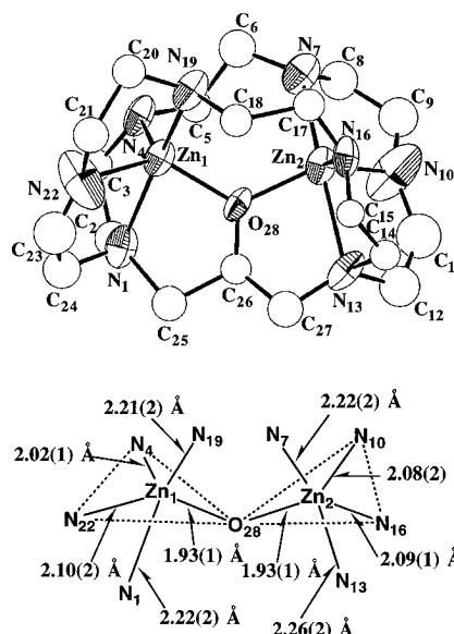
Figure 3. Crystal structure of 8 and its coordination bonding scheme with three perchlorates omitted for clarity. Thermal ellipsoids for zinc, nitrogen and oxygen atoms and circles for carbon atoms are at 30% probability level. Bond angles (deg) around zinc(II) ions are as follows: O 28 -Zn 1 -N 1 , 79.2(6); O 28 -Zn 1 -N 4 , 103.1(6); O 28 -Zn 1 -N 19 , 100.7(5); O 28 -Zn 1 -N 22 , 130.8(9); N 1 -Zn 1 -N 4 , 84.9(7); N 1 -Zn 1 -N 19 , 159.0(6); N 1 -Zn 1 -N 22 , 80.2(9); N 4 -Zn 1 -N 19 , 115.2(7); N 4 -Zn 1 -N 22 , 118.8(9); N 19 -Zn 1 -N 22 , 84.4(9); O 28 -Zn 2 -N 7 , 102.9(6); O 28 -Zn 2 -N 10 , 130.6(9); O 28 -Zn 2 -N 13 , 77.7(6); O 28 -Zn 2 -N 16 , 101.8(6); N 7 -Zn 2 -N 10 , 82.5(10); N 7 -Zn 2 -N 13 , 159.3(6); N 7 -Zn 2 -N 16 , 115.6(7); N 10 -Zn 2 -N 13 , 81.8(10); N 10 -Zn 2 -N 16 , 120.2(9); N 13 -Zn 2 -N 16 , 84.0(7).
