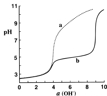
Figure 1. Typical titration curves for propanol-bridged octaazacryptand 7 at 35 °C with I = 0.10 ( \text{NaNO}_3 ): (a) 1.0 mM 7 ·8HCl; (b) a + 2.0 mM \text{Zn}^{\text{II}}\text{SO}_4 . a(\text{OH}^-) is the number of equivalents of base added.
