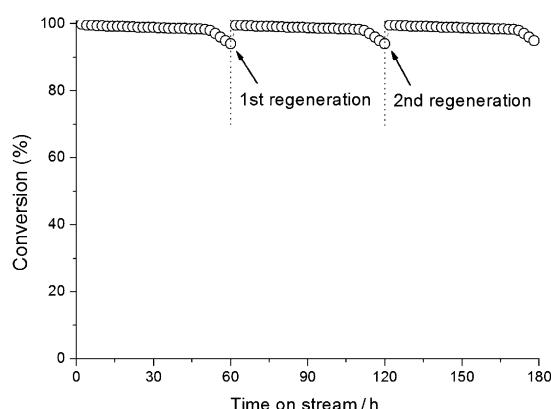
Figure 3. Long-term performance of dehydration of aqueous 1-PO (50 wt %) over HZSM-5-30. Reaction conditions: 2.0 g HZSM-5-30, 250^\circ\text{C} , 50 wt % aqueous 1-PO feedstock, \text{WHSV} = 1.0 \text{ h}^{-1} , at atmosphere pressure, \text{N}_2 flow rate 20 \text{ mL min}^{-1} , selectivity to propylene always > 99\% .
