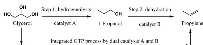
Scheme 1. Catalytic conversion of glycerol to propylene (GTP).
