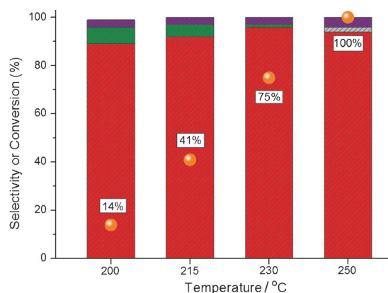
Figure 2. Catalytic hydrogenolysis of aqueous glycerol (10 wt%) over 1 wt% Ir/ZrO 2 performed at different temperatures. Reaction conditions: glycerol 1.0 g, Ir/ZrO 2 (Ir 0.12 mol%), 4 h, 5 MPa H 2 (RT). Selectivity: ■ gas, ■ MeOH, ■ EtOH, ■ EG, ■ 1,3-PDO, ■ 1,2-PDO, ■ 1-PO; conversion: ● glycerol.
