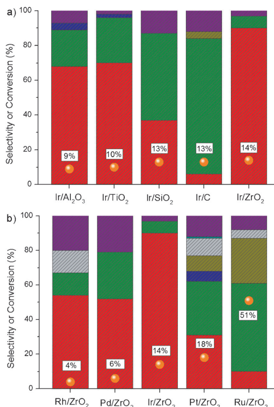
Figure 1. Catalytic hydrogenolysis of aqueous glycerol (10 wt%) over a) 1 wt% Ir supported on different oxides; and b) various noble metals loaded on ZrO 2 . Reaction conditions: glycerol 1.0 g, metal 0.12 mol%, 200 °C, 4 h, 5 MPa H 2 (RT). Selectivity: ■ gas, ■ MeOH, ■ EtOH, ■ EG, ■ 1,3-PDO, ■ 1,2-PDO, ■ 1-PO; conversion: ● glycerol.
