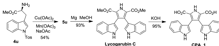
Scheme 5. Biomimetic Synthesis of Lycogarubin C and CPA
