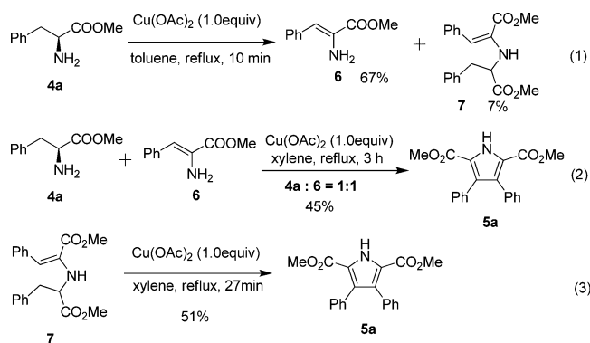
Scheme 3. Studies on the Reaction Mechanism
