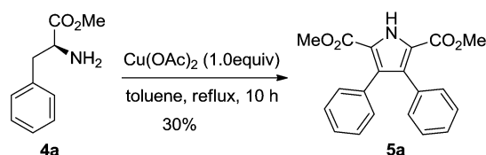
C \text{Cu}(\text{OAc})_2 promoted oxidation cyclization for the synthesis to pyrrole 5a
