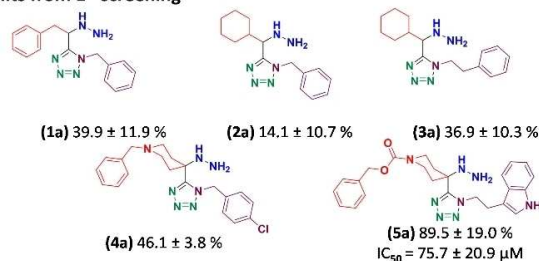
Figure 3. Chemistry and first hits. A) Design of an MCR incorporating hydrazine. B) Structures and % inhibition – IC 50 values of initial hits (set 1).
