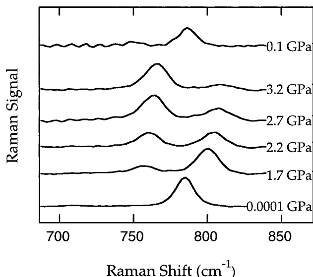
Figure 1. Raman spectra of a solution of acetone and methanol dissolved in tetrahydrofuran reveal reversible spectral changes attributed to pressure induced hemiketal formation. Spectra were collected over a series of increasing pressures followed by a pressure decrease (spectra are shifted vertically for clarity). The C–C stretch of acetone at \sim 780 \text{cm}^{-1} shifts to 800 \text{cm}^{-1} with increasing pressure, as the hemiketal C–C peak grows in at \sim 760 \text{cm}^{-1} .
