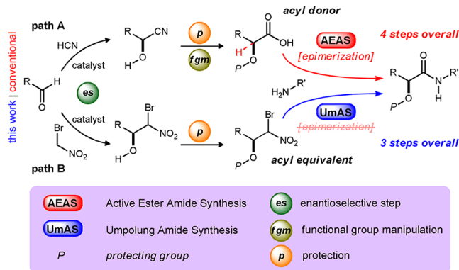
Figure 1. Comparison of conventional \alpha -oxy amide synthesis approaches to the Henry/UmAS method used in this work.
