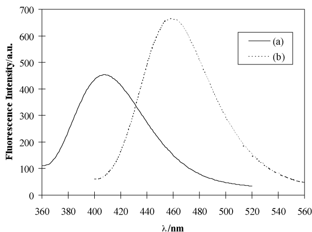
Figure 2. Fluorescence spectra of (a) Glt-Phe-NH-ca-OEt ( 8 ); \lambda_{\text{ex}} =341 nm, (b) Aca-OEt ( 3 ); \lambda_{\text{ex}} =366 nm. 1 \mu\text{M} solutions in 0.05 M Tris-HCl, pH 7.8, containing 1% DMSO.
