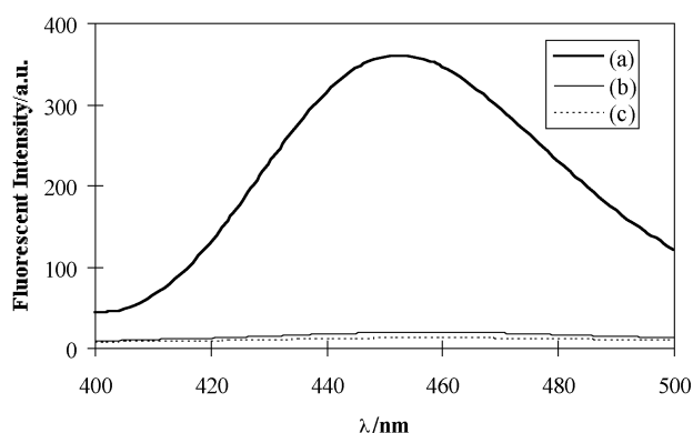
Figure 3. Fluorescence spectra of (a) Hca ( 2 ); \lambda_{\text{ex}} =350 nm, (b) Ole-Oca ( 13 ), (c) Pal-Oca ( 14 ); \lambda_{\text{ex}} =368 nm. 1 \mu\text{M} solutions in 0.05 M Tris-HCl, pH 7.8, containing 1% DMSO.
