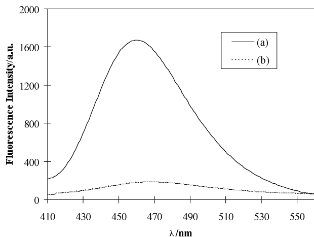
Figure 1. Fluorescence spectra of (a) Aca-Phe-OH ( 6 ), (b) Aca-Phe-NH-Np ( 5 ); \lambda_{\text{ex}} =364 nm. 1 \mu\text{M} solutions in 0.05 M Tris-HCl, pH 7.8, containing 1% DMSO.
