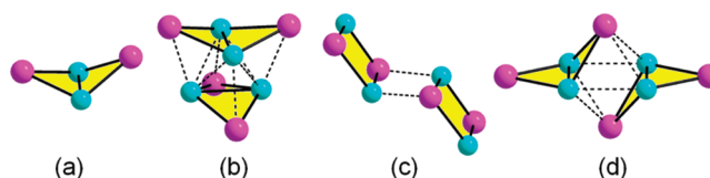
Figure 1. Illustrations of the copper iodide cores of (a) Cu 2 I 2 cluster, (b) cubane-like Cu 4 I 4 cluster, (c) repeat unit of a staircase (CuIL) ∞ cluster, and (d) a new type of Cu 4 I 4 cluster, based on crystallographic structural data, Cu, cyan; I, purple. The solid lines show the bonding within the Cu 2 I 2 fragment, and the dashed lines in (b), (c), and (d) illustrate the bonding between Cu 2 I 2 fragments (based on close atom–atom contacts in the crystal structures).
