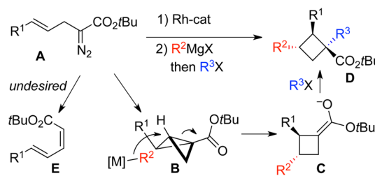
Scheme 1. Multicomponent Cyclobutane Synthesis
