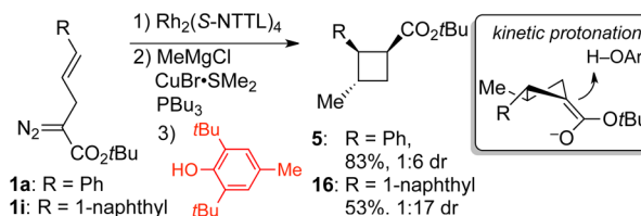
Scheme 2. Reversal of Diastereoselectivity
