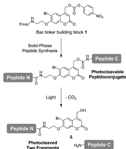
Fig. 1 Schematic illustration of synthesis and photochemistry of photocleavable peptidoconjugates containing the Bac linker.
