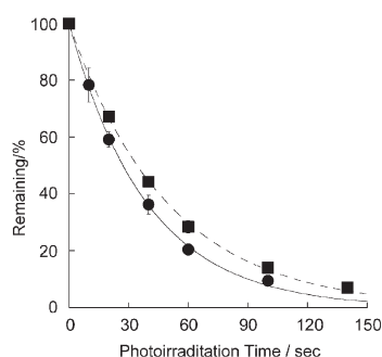
Fig. 4 Time courses of photolysis of peptidoconjugates 5 ( \bullet , 9 \mu M) and 6 ( \blacksquare , 8 \mu M) in K-MOPS buffer.
