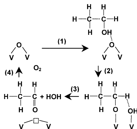
Figure 3. Proposed scheme for ethanol oxidation to ethanal.
