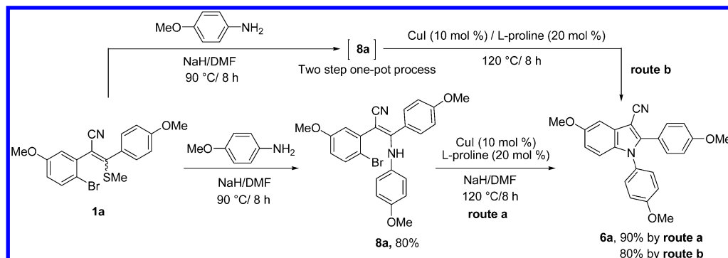
Scheme 4. Synthesis of Indole 6a from 1a via Enaminonitrile 8a
