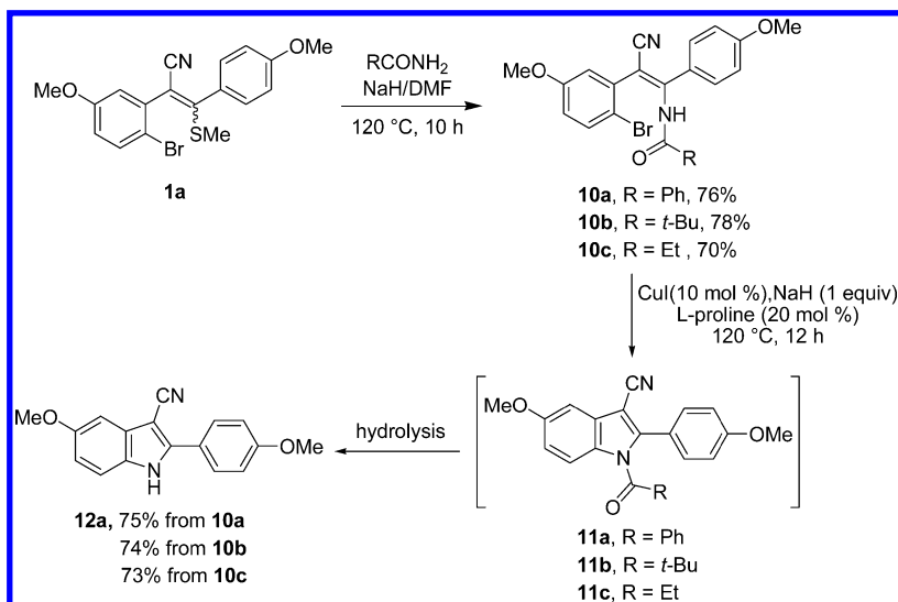
Scheme 5. Synthesis of N -Acylenaminonitriles and Their Cu-Catalyzed Intramolecular N -Arylation–Hydrolysis to Indole 12a
