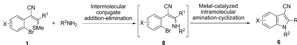
Scheme 4. Synthesis of Indole 6a from 1a via Enaminonitrile 8a
