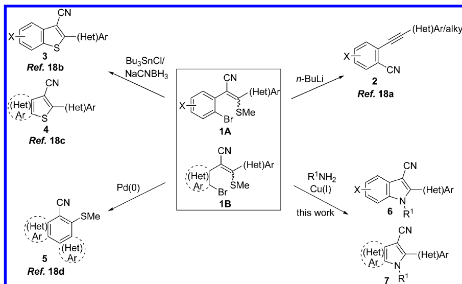
Scheme 1. 2-[2-Bromo(het)aryl]-3-(het)aryl-3-(methylthio)acrylonitriles as Versatile Synthons for Heterocyclic Synthesis
