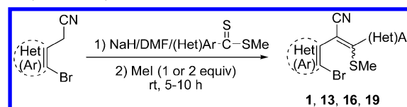
Scheme 2. Synthesis of 2-[2-Bromo(het)aryl]-3-(het)aryl-3-(methylthio)acrylonitrile Precursors
