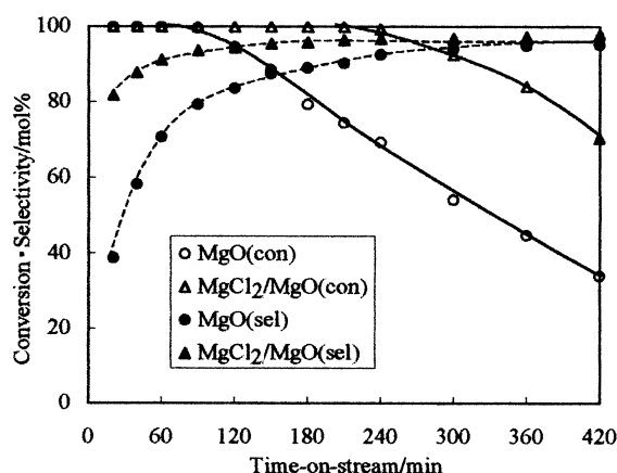
(con : conversion, sel : selectivity) Figure 1. Effect of \text{MgCl}_2 on the vapor-phase hydrogen transfer reaction over \text{MgO} -based catalysts. reaction temperature : 270 °C, contact time : 28.8 g-cat h/mol, nitrogen flow rate : 10 L/h.
