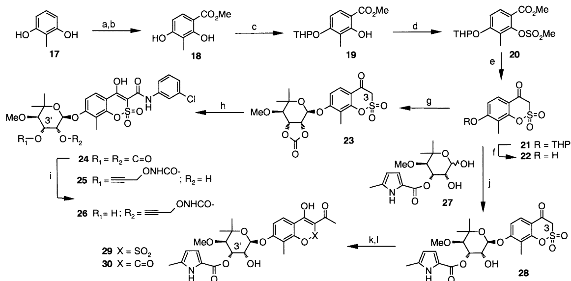
Scheme 2. Reagents and conditions: (a) DMF, POCl 3 , ClCH 2 CH 2 Cl, rt, 73%; (b) MnO 2 , KCN, AcOH, MeOH, rt, 68%; (c) DHP, cat TsOH, Et 2 O, rt, 71%; (d) MsCl, Et 3 N, Et 2 O, rt, 90%; (e) NaH, DMF, 0°C, 82%; (f) 1 M HCl in MeOH, rt, 86%; (g) 11 , BF 3 ·Et 2 O, CH 2 Cl 2 , 50%; (h) 3-ClC 6 H 4 -NCO, DMAP, CH 2 Cl 2 , rt, 23%; (i) HC≡CCH 2 ONH 2 -HCl, LiClO 4 , Py, rt, 64%; (j) PPh 3 , EtO 2 CN=NCO 2 Et, CH 2 Cl 2 , rt, 15%; (k) Ac 2 O, DMAP, CH 2 Cl 2 , rt; (l) KOMe, MeOH, 0°C, 37% (from 27 )
