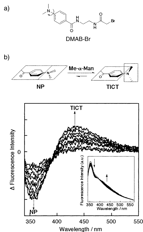
Figure 7. a) Structure of DMAB-Br. b) Differential spectral changes in the fluorescence of DMAB-Con A upon addition of Me- \alpha -Man (0 → 10 mM). [DMAB-Con A] = 1 \mu M in 50 mM HEPES buffer (pH 7.0) containing 1 mM CaCl 2 , 1 mM MnCl 2 , and 0.1 M NaCl. Temperature = 15 \pm 1 ^{\circ} C, \lambda_{ex} = 310 nm. Inset: fluorescence spectral changes.
