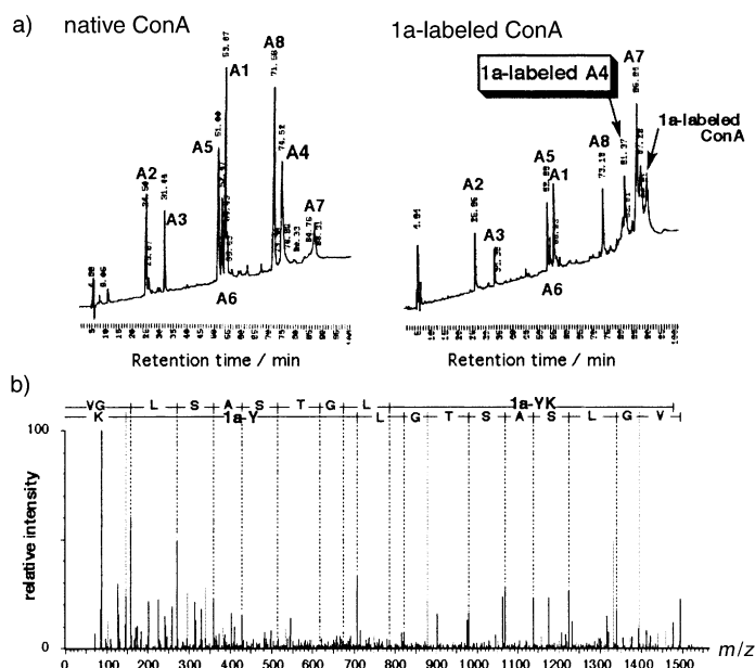
Figure 4. a) Reverse-phase HPLC trace of native and 1a -labeled Con As after lysyl-endopeptidase digestion. b) Tandem mass–mass analysis of the 1a -labeled fragment A4.
