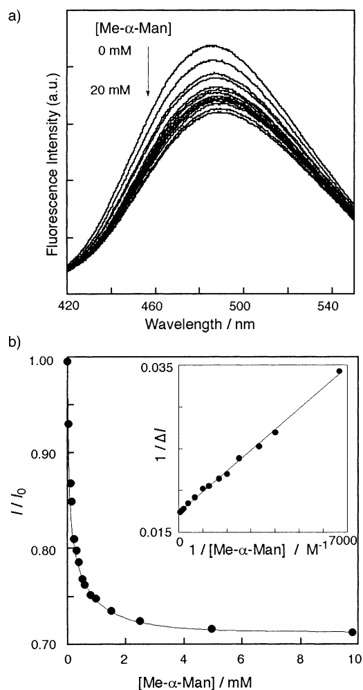
Figure 5. a) Spectral changes in the fluorescence of IAEDANS-Con A upon addition of Me- \alpha -Man (0 \rightarrow 20 mM). [IAEDANS-Con A] = 5 \mu\text{M} , in 50 mM HEPES buffer (pH 7.0) containing 1 mM \text{CaCl}_2 , 1 mM \text{MnCl}_2 , and 0.1 M NaCl. Temperature = 15 \pm 1^\circ\text{C} , \lambda_{\text{ex}} = 340 nm. b) The binding curve for IAEDANS-Con A. Inset: Benesi–Hildebrand plot analysis. HEPES = 2-[4-(2-hydroxyethyl)-1-piperazinyl]ethanesulfonic acid.
