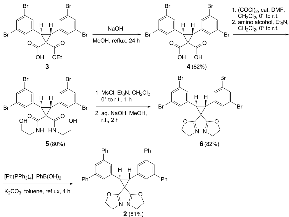
Scheme. Synthesis of Bis[dihydrooxazole] Ligand 2
