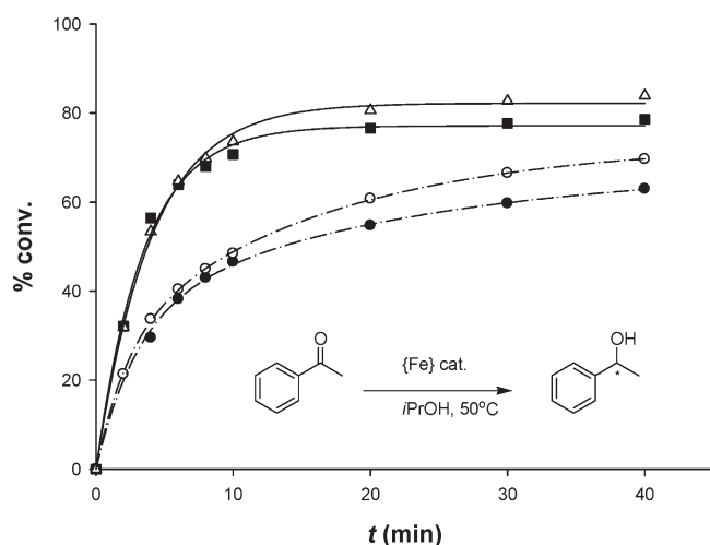
Figure 4. Catalytic transfer hydrogenation of acetophenone to 1-phenylethanol in isopropanol at 50 °C in the presence of (■) (S,S)- 1f , KOtBu (catalyst/base/substrate = 1/8/500) (see ref 9); (Δ) (S,S)- 2f (catalyst/substrate = 1/500); (●) 1e , KOtBu (catalyst/base/substrate = 1/8/200) (see ref 9); (○) 2e (catalyst/substrate = 1/200).
