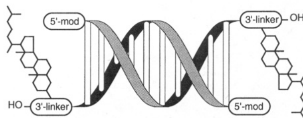
Figure 1. Schematic structure of the 3'-cholesterol-modified DNA duplexes.
