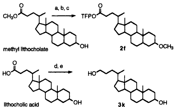
Scheme 2. Synthesis of Lithocholic Acid Intermediates a
