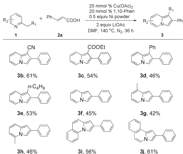
Scheme 1. Scope of the Synthesis of Indolizines: Substituents on 2-Alkylazaarenes a
