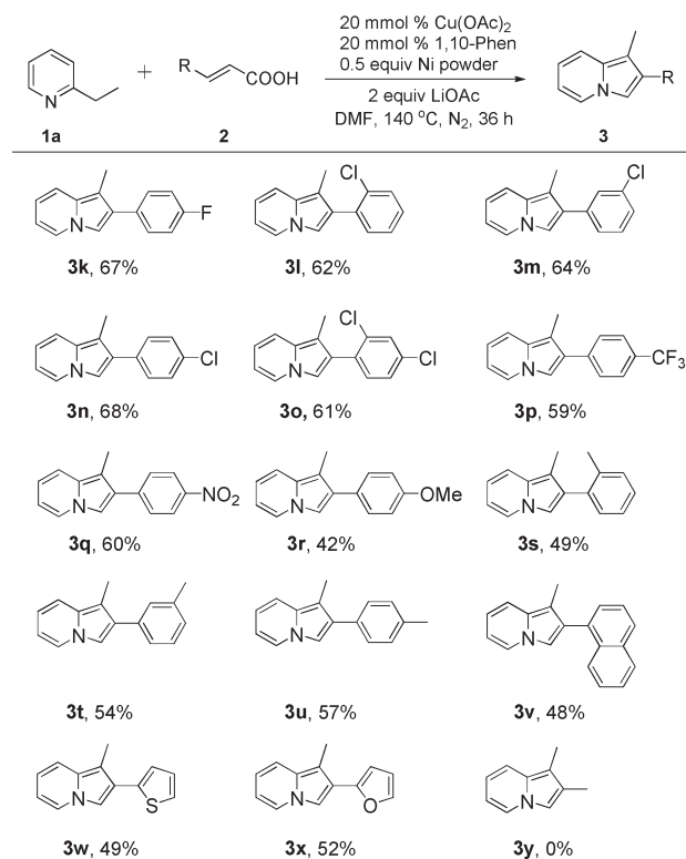
Scheme 2. Scope of the Synthesis of Indolizines: Substituents on \alpha,\beta -Unsaturated Carboxylic Acids a
