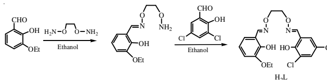
Scheme-I: Synthetic route to 6-ethoxy-4',6'-dichloro-2,2'-[ethylenedioxybis(nitrilomethylidyne)]diphenol ( H_2L )
