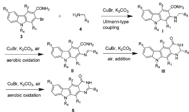
Scheme 2 Possible mechanism.
