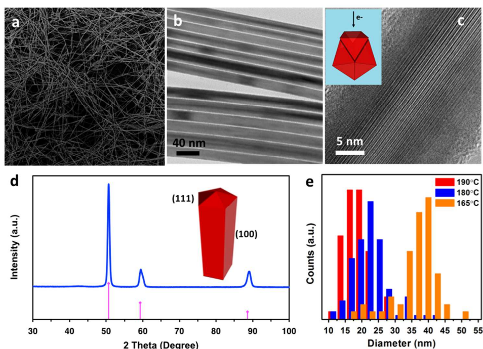
Figure 2. (a) SEM and (b) TEM and (c) HRTEM images of as synthesized Cu NW at 190 °C. (d) XRD pattern of as made Cu NWs, inset is a schematic representation of the NW's micro structure. Pink lines are the standard XRD pattern of FCC copper. (e) Diameter distribution of Cu NWs synthesized at 190 °C (red), 180 °C (blue), and 165 °C (orange).
