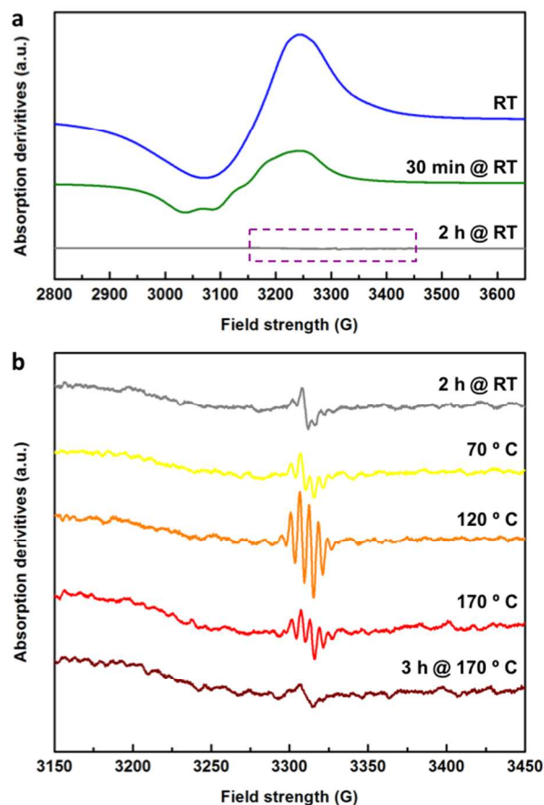
Figure 3. (a) In-situ EPR response of the reactants at RT. From the top, it shows the reactant' EPR signals upon mixing (blue), after 30 mins at RT (green) and 2 hours after RT (grey). (b) EPR signals of the reaction during heating. From the top, it shows EPR spectra of the reaction before heating (grey, the enlarged purple area in Fig. 3a), at 70 °C (yellow), at 120 °C (orange), at 170 °C (red), and 3 hours at 170 °C (wine).
