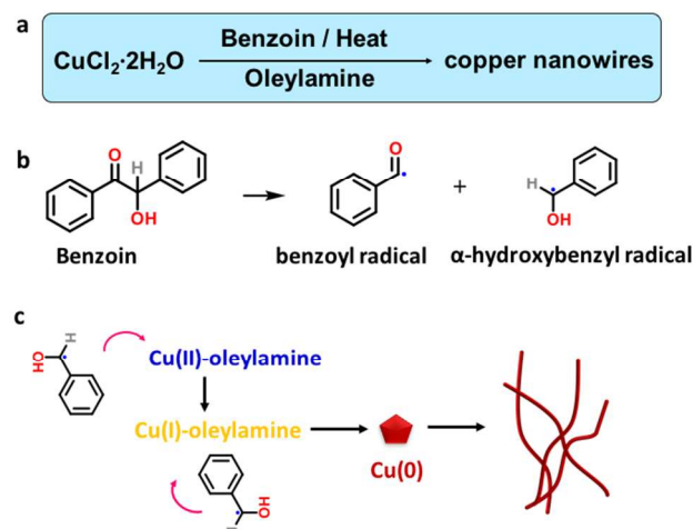
Figure 1. (a) Overall reaction scheme of Cu NW synthesis using benzoin as reducing agents. (b) Heat induced radical generation
