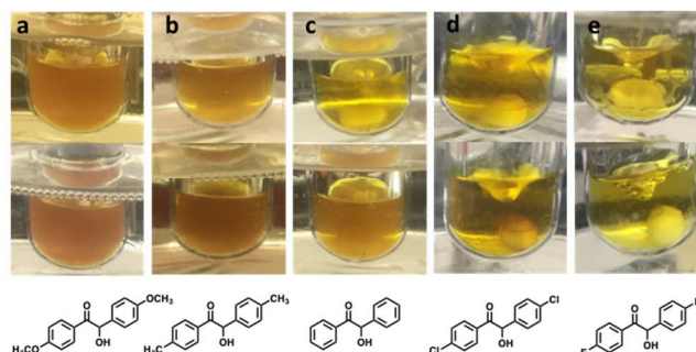
Figure 4. Pictures of different stages of Cu NWs synthesis using (a), 4,4-dimethoxybenzoin; (b), 4,4-dimethylbenzoin; (c), benzoin; (d), 4,4-dichlorobenzoin 22 and (e), 4,4-difluorobenzoin 22 as reducing agents. The upper and middle panel show the pictures of reactions run for 1 hour and 2 hours respectively; the lower panel shows the chemical structures used in corresponding reactions. The reactions were all carried out at 180 °C.
