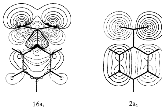
Figure 4. 16a 1 (σ) (SOMO) and 2a 2 (π) (the second HOMO).
