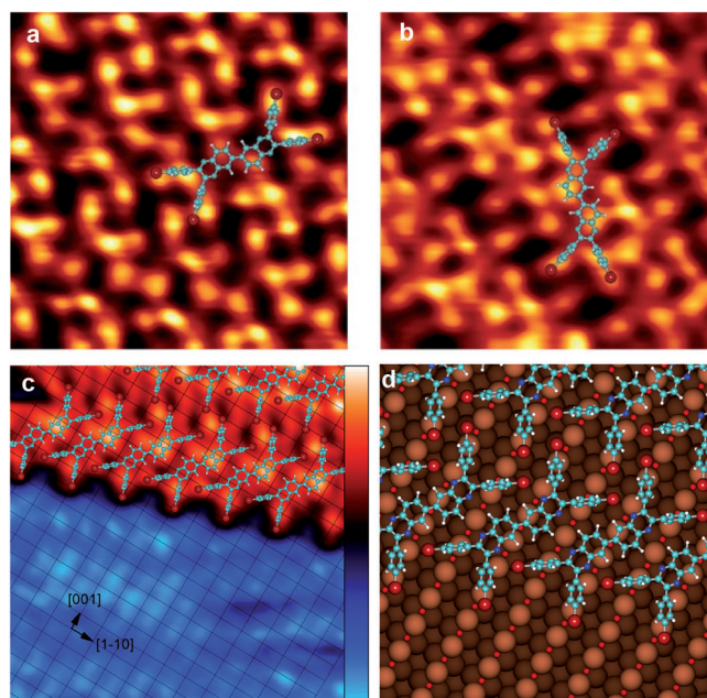
Figure 3. STM images that show the chirality of the TBPBQ domains: a) 5.1 \times 5.1 nm 2 , b) 5 \times 5 nm 2 ( U_s = -1.42 V, I_t = 0.7 nA). c) Determination of the adsorption site of the molecules on the surface (7.7 \times 8 nm 2 , U_s = -0.74 V, I_t = 0.77 nA). d) Tentative structural model of adsorbed TBPBQ molecules on the Cu(110)-O(2 \times 1) surface.
