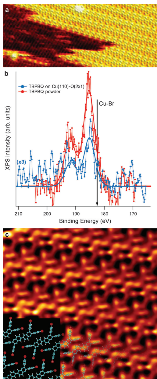
Figure 2. a) STM images of TBPBQ/Cu(110)-O(2 \times 1) with atomic resolution (30 \times 12 nm 2 , U_s = -0.74 V, I_t = 0.77 nA). b) XPS Br 3p core-level spectra of TBPBQ powder (red) and TBPBQ on Cu(110)-O(2 \times 1) (blue). c) High-resolution STM image of TBPBQ on Cu(110)-O(2 \times 1) at 150 K (7 \times 7 nm 2 , U_s = -1.42 V, I_t = 0.74 nA).
