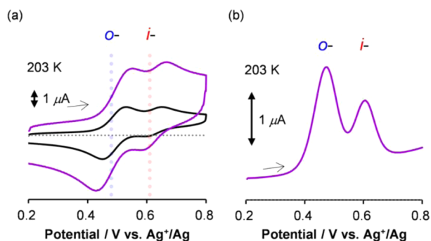
Figure 3. (a) Cyclic voltammograms of 1^+\text{BF}_4^- (0.45 mM) in 0.1 M \text{Bu}_4\text{N}^+\text{BF}_4^- - \text{CH}_2\text{Cl}_2 at a scan rate of 250 (purple line) and 50 \text{mV s}^{-1} (black line) at 203 K. (b) Differential pulse voltammogram under the same conditions as for part a.
