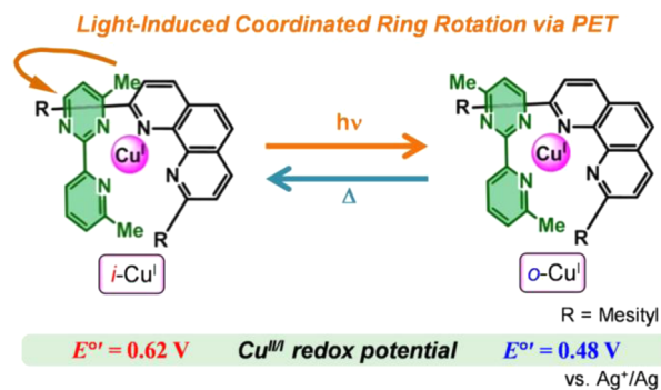
Figure 1. Conceptual diagram showing the photodriven and heat-driven pyrimidine ring rotational isomerization of 1^+BF_4^- .
