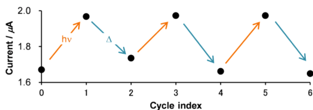
Figure 8. Changes in the anodic peak current at 0.55 V in the experimental cyclic voltammograms of \text{I}^+\text{BF}_4^- (0.45 mM) in 0.1 M \text{Bu}_4\text{N}^+\text{BF}_4^- – \text{CH}_2\text{Cl}_2 containing 1.8 mM \text{DMFc}^+\text{BF}_4^- at 203 K.
