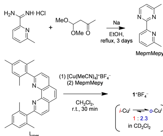
Scheme 1. Synthesis of 1^+BF_4^-
