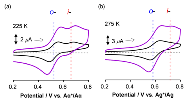
Figure 4. Cyclic voltammograms of 1^+\text{BF}_4^- (0.45 mM) in 0.1 M \text{Bu}_4\text{N}^+\text{BF}_4^- - \text{CH}_2\text{Cl}_2 at a scan rate of 250 (purple line) and 50 \text{mV s}^{-1} (black line) at 225 K (a) and 275 K (b) in the dark.
