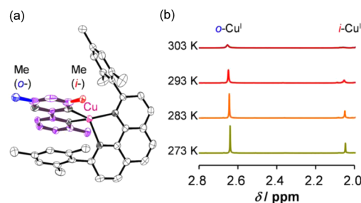
Figure 2. (a) ORTEP view of 1^+BF_4^- \cdot CH_2Cl_2 \cdot 0.5 hexane. The displacement ellipsoids are drawn at a 50% probability level. Hydrogen atoms, counteranions, crystal solvents, and one complex cation are omitted for clarity. (b) Temperature dependence of the methyl signal on the pyrimidine moiety in the ^1H NMR spectrum in CD_2Cl_2 in the dark.
