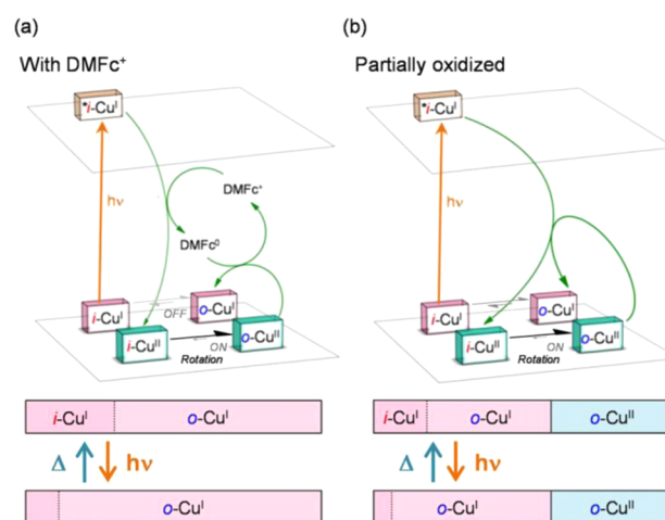
Figure 9. (a, b) Schematic representation of the PET-driven i -Cu I to o -Cu I ligand geometry isomerization of (a) \text{I}^+\text{BF}_4^- in the presence of \text{DMFc}^+ and (b) the partial oxidation of \text{I}^+\text{BF}_4^- by (\text{NH}_4)_2[\text{Ce}(\text{NO}_3)_6]^{2-} . The reversible changes in the molar ratios of the isomers upon light irradiation and heating are illustrated in the bottom panels.
