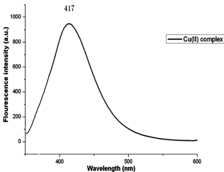
Figure 7. Emission spectrum of the Cu(II) complex in dilute DMF at room temperature ( c = 5 \times 10^{-5} \text{ mol L}^{-1} , \lambda_{\text{em}} = 417 \text{ nm} ).
