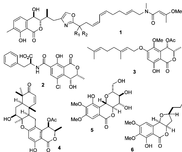
Figure 1. Isochromone-containing natural products.
