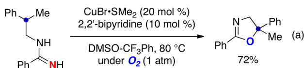
Scheme 1. Oxidative Functionalization of C–H Bonds, Alkenes, and Alkynes with an Amidine Moiety
