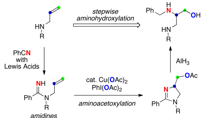
Scheme 2. Synthesis of 4-Acetoxymethyl-4,5-dihydroimidazoles via Aminoacetoxylation of Alkenes and Their Conversion to 2,3-Diamino-1-propanols: Stepwise Strategy on Regioselective Aminoacetoxylation of Allylamine (This Work)
