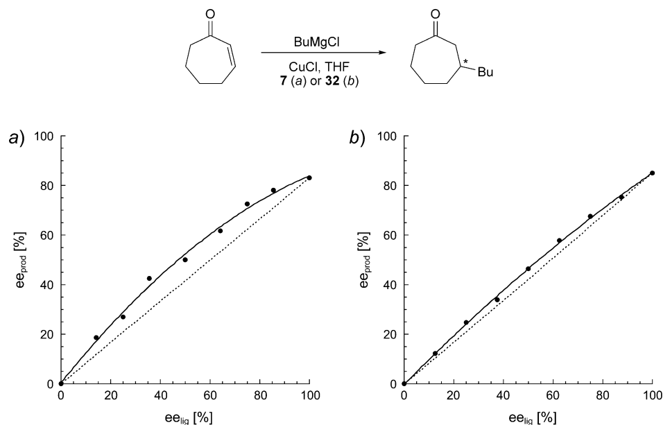
Fig. 4. Positive nonlinear effect (NLE) for the Cu-catalyzed 1,4-addition of BuMgCl to cycloheptenone using ligand 7 (a) and ligand 32 (b). The reactions were carried out under the conditions specified in Table 4 and in the accompanying text.
