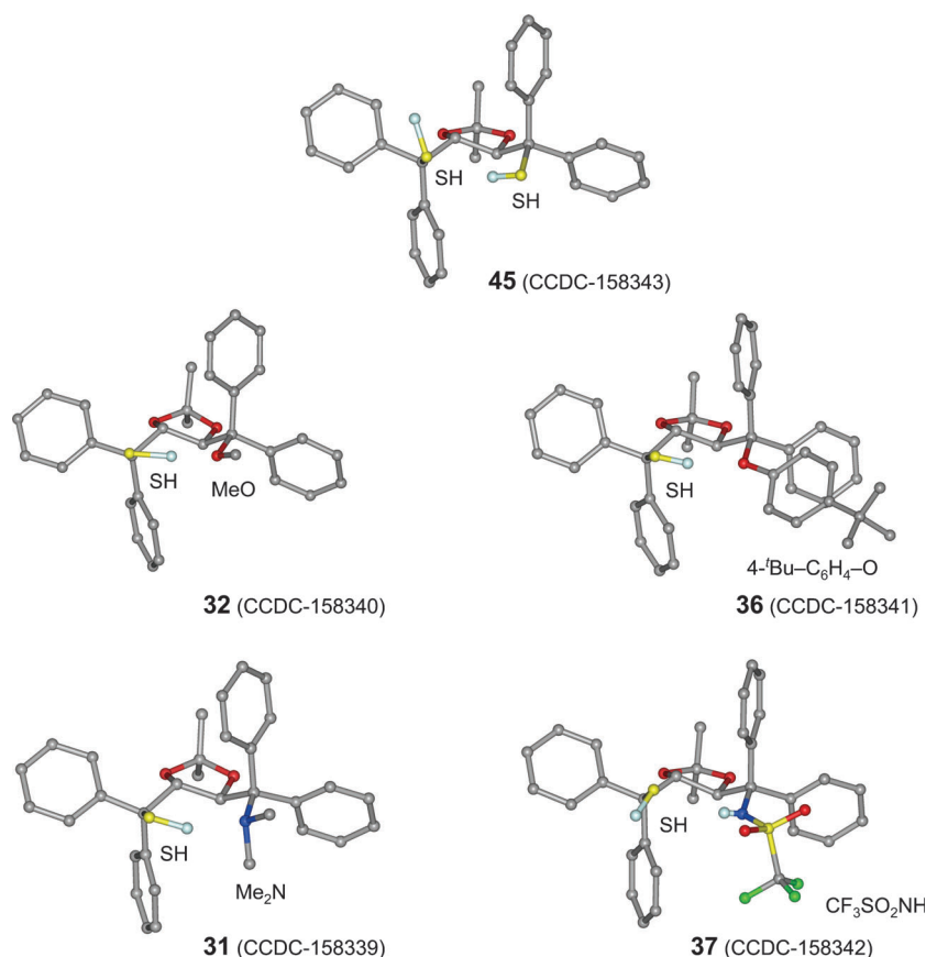
Fig. 2. X-Ray crystal structures of the five sulfanyl derivatives 31, 32, 36, 37, and 45 with the CCDC codes. There are H-bonds between the SH groups and a heteroatom S, O, or N, in seven-membered H-bonded rings. In 37 , the \text{CF}_3\text{SO}_2\text{NH} H-atom acts as the H-bond donor. The heteroatoms on all exocyclic C,C bonds are antiperiplanar to each other, i.e. , not in the stereoelectronically more favorable gauche -conformation.
