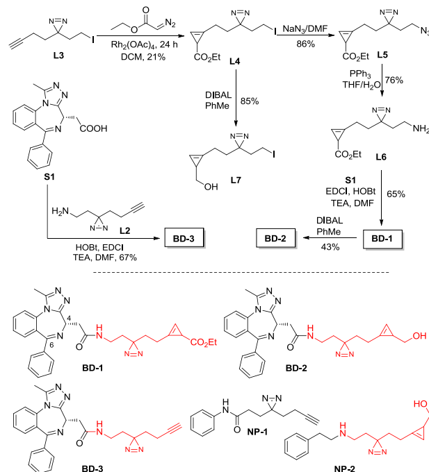
Scheme 1. Synthesis of Diazirine Containing Cyclopropene Linkers (L4/L7) and BRD-4 Targeting Probes (BD-1/3).
