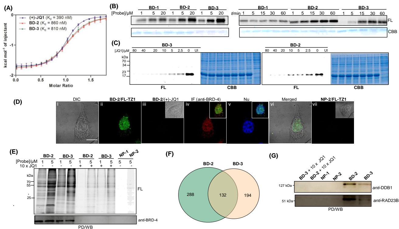
Figure 3. (A) ITC results of (+)-JQ1/ BD-2/BD-3 binding to (His) 6 -tagged BRD-4. See Figure S12 for details. (B) Concentration-dependent labeling of BD-1/2/3 with recombinant BRD-4 (2 \mu g; left gels), and time-dependent ligation (1 to 60 min; 5 \mu M probe) of probe-labeled BRD-4 with TER-TZ1 (for BD-1/2 ) and TER-N 3 (for BD-3 ). FL = in-gel fluorescence scanning. CBB = Coomassie gel. (C) Labeling of (His) 6 -tagged BRD-4 over-expressing bacterial lysates by 1 \mu M of BD-3 (left gels) or BD-2 (right gels), in the presence of different amounts of (+)-JQ1 (0–80 \mu M), with TER-TZ1 (10 \mu M; 2 h ligation). (D) Live-cell imaging of BD-2/NP-2 (5 \mu M) followed by ligation with FL-TZ1 . IF = immunofluorescence. Merged: panels i + ii. (Insets in panels iv & v): merged panels ii/iv (with a Pearson's coefficient R = 0.76 ) & ii/v, respectively. Scale bar = 10 \mu m. (E) In-gel fluorescence scanning showing the proteome reactivity profiles of live HepG2 cells labeled by BD-2/BD-3 , with or without 10 x (+)-JQ1. The corresponding pull-down (PD)/Western blotting (WB) results are shown (bottom gel). For BD-2 -labeled cells, ligation was done with TER-TZ1/Biotin-TZ2 . NP-1/NP-2 : negative control PD. (F) Venn diagram showing the number of proteins labeled/enriched by BD-2/3 (1 \mu M) upon in situ labeling/PD/LC-MS/MS with live HepG2 cells. Non-specific protein labeling was minimized by control labeling experiments with NP probes, and with 10 x (+)-JQ1. (G) Preliminary validation of the two newly identified off-targets of (+)-JQ1 by PD/WB from BD-2 (1 \mu M)-labeled HepG2 cells. BD-3 labeling was carried out concurrently as a reference. The corresponding control experiments were done with negative probes ( NP-1 & NP-2 ) and with 10 x (+)-JQ1.
