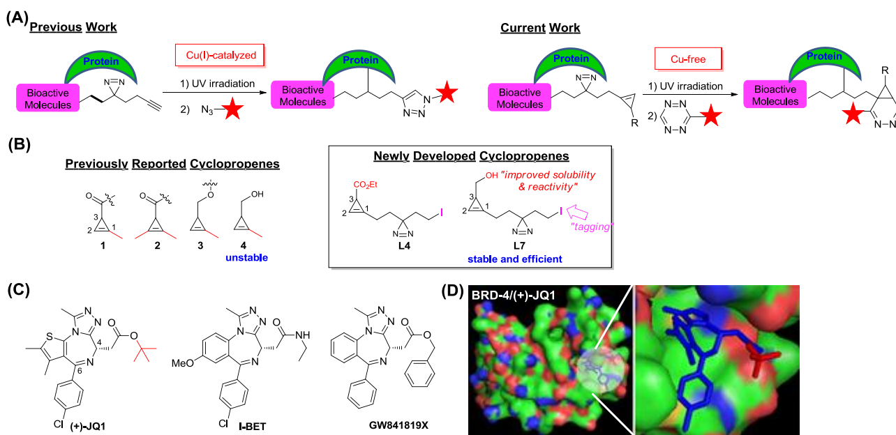
Figure 1. (A) Two drug-profiling PAL approaches: (left) previously developed approach in which bioactive compounds were “tagged” with 1 st -generation “minimalist” linkers; 9 (right) 2 nd -generation approach reported in the current work, with cyclopropenes as chemically tractable tags suitable for copper-free bioorthogonal chemistry. (B) Structures of previously reported cyclopropenes ( 1-4 ), 18-20 and newly reported ones ( L4 & L7 ; boxed). (C) Known BRD-4-targeting compounds. (D) the x-ray complex (PDB code: 3MXF) of BRD-4/(+)-JQ1 showing the active-site binding (right panel). 24a
