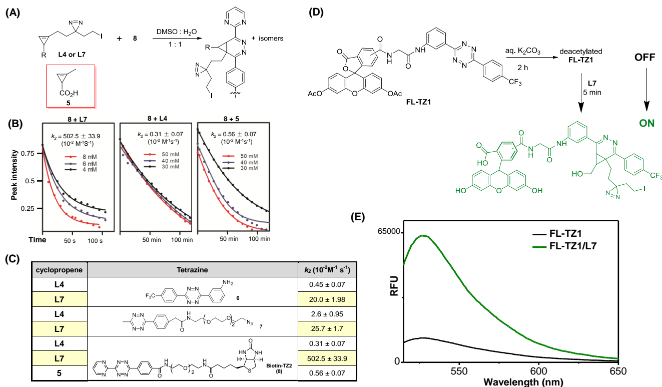
Figure 2. (A) Scheme of tetrazine 8 reacting with cyclopropene L4 , L7 or 5 . Different diazonorcaradiene regioisomeric products could form, but for simplicity, only one regioisomer is depicted. (B) Plots of tetrazine absorbance (520 nm) versus time between ligation of 8 and L7 , L4 or 5 . Data was fitted to a first-order exponential decay to obtain the corresponding second-order rate constant ( k_2 ). (C) k_2 of different tetrazines 6 , 7 or 8 reacting with L7 , L4 or 5 . (D) Schematic showing of ligation reaction between FL-TZ1 and L7 . (E) Emission spectra of deacetylated FL-TZ1 alone, and 5 min after ligation with L7 . 10 \mu\text{L} of FL-TZ1 (10 mM in DMSO) was first treated with 20 \mu\text{L} \text{K}_2\text{CO}_3 solution (100 mM) for 2 h at room temperature. Next, 40 \mu\text{L} L7 (15 mM in 10% DMSO/ \text{H}_2\text{O} ) was added and the reaction mixture was incubated for 5 min. Upon dilution (500 x with 10% DMSO/ \text{H}_2\text{O} ), the emission fluorescence was measured ( \lambda_{\text{ex}} = 488 \text{ nm} ). Control sample was processed under the same conditions without addition of L7 .
