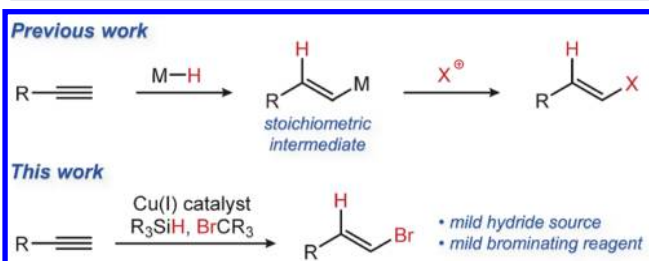
Figure 1. Anti-Markovnikov Hydrohalogenation of Alkynes.
