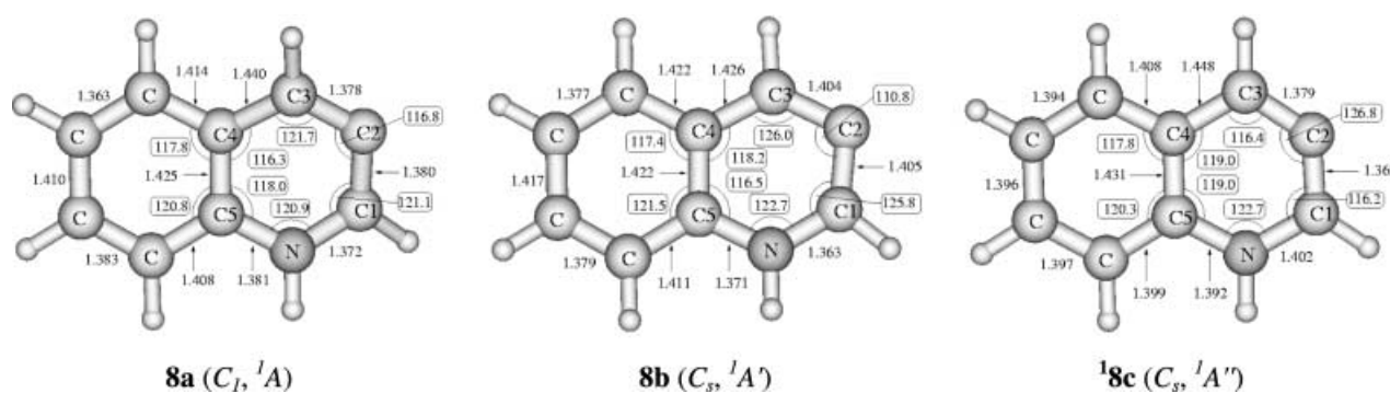
Figure 3. Optimised C–C and C–N bond lengths [Å] and bond angles [°] computed [B3LYP/6–31G(d)] for various stationary points of 3\delta^2 -1H-quinoline ( 8 ).
