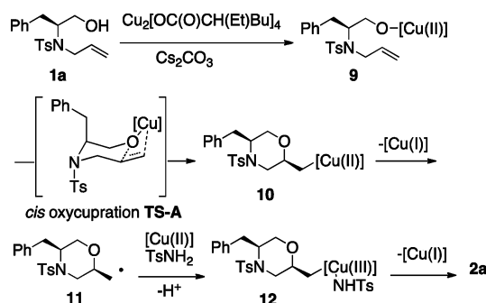
Scheme 2. Proposed Oxyamination Reaction Mechanism
