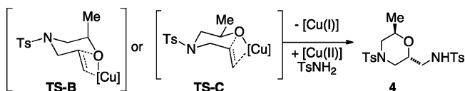
Scheme 3. Rationalization of 2,6- trans -Selectivity
