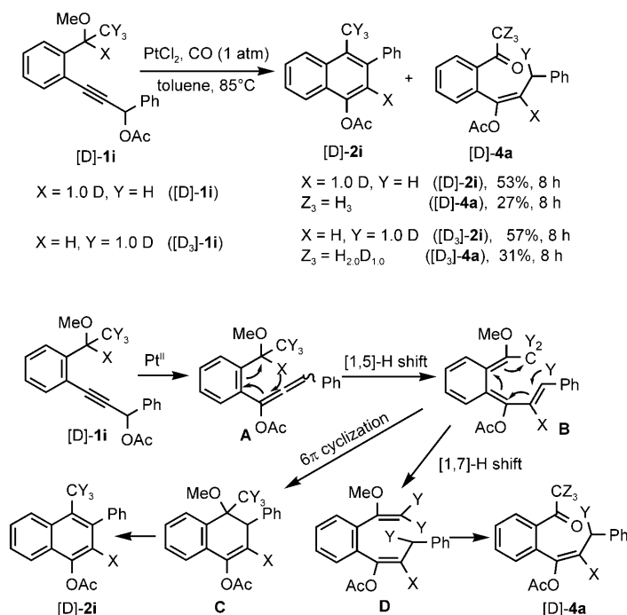
Scheme 1. Deuterium-labeling experiments and proposed mechanism.
