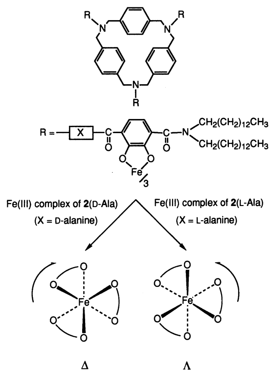
Fig. 2. Absolute configurations of iron(III) complexes of 2 (L-Ala) and 2 (D-Ala).
