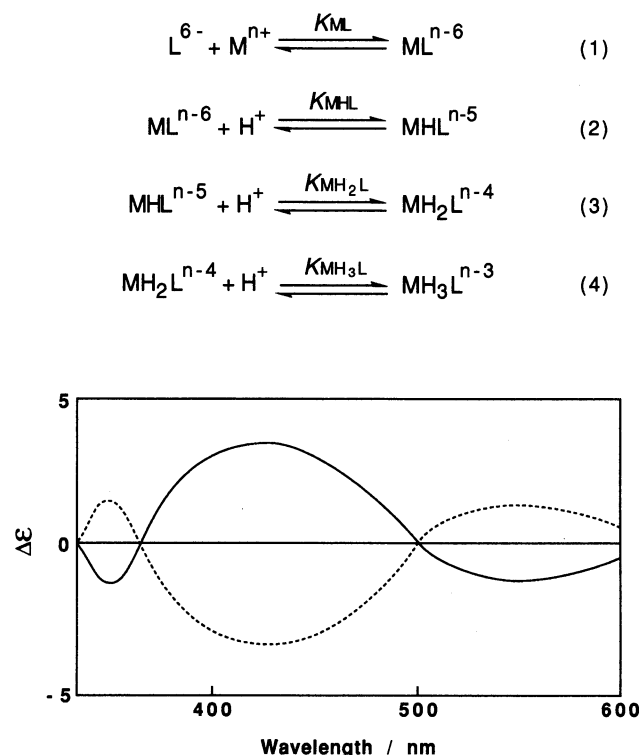
Fig. 1. CD spectra of iron(III) complexes of 2 (L-Ala) (—) and 2 (D-Ala) (---) in Tris buffer (pH 9.0) at 30.0 °C.
